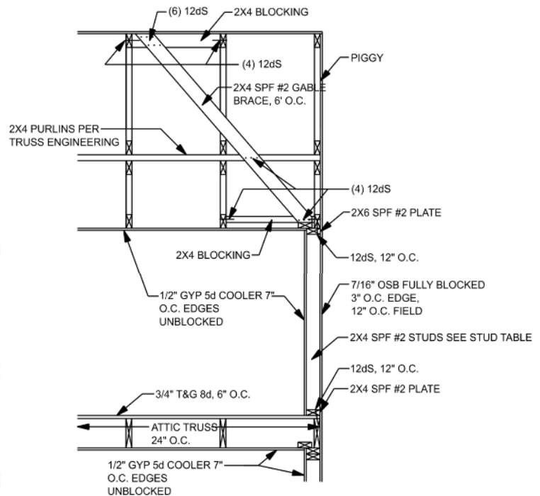
BONUS ROOM / GABLE END BRACING
