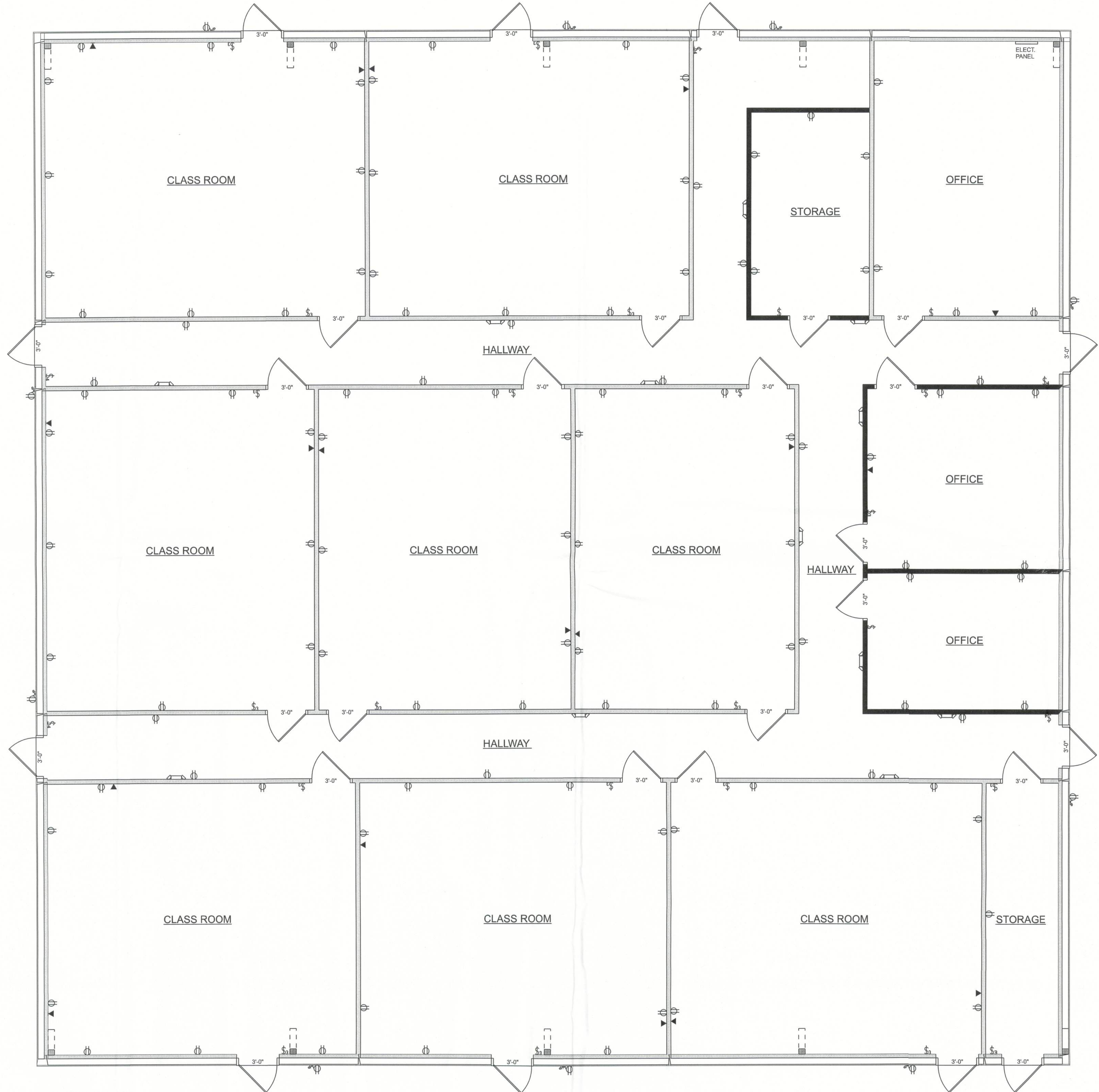
POWER PLAN SCALE: 1/4" = 1'-0"
