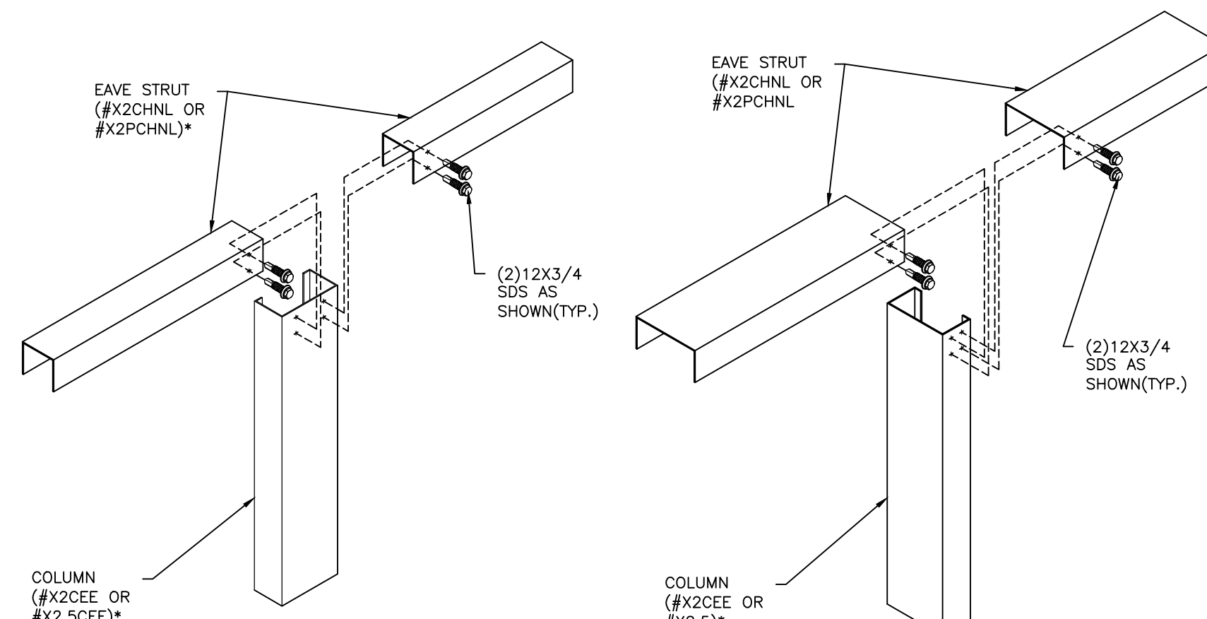
DIVIDER PARTITION WALL FRAMING DETAIL CONDITION 2 FRAMING GAUGES SPECIFIED ON BUILDING DRAWINGS
