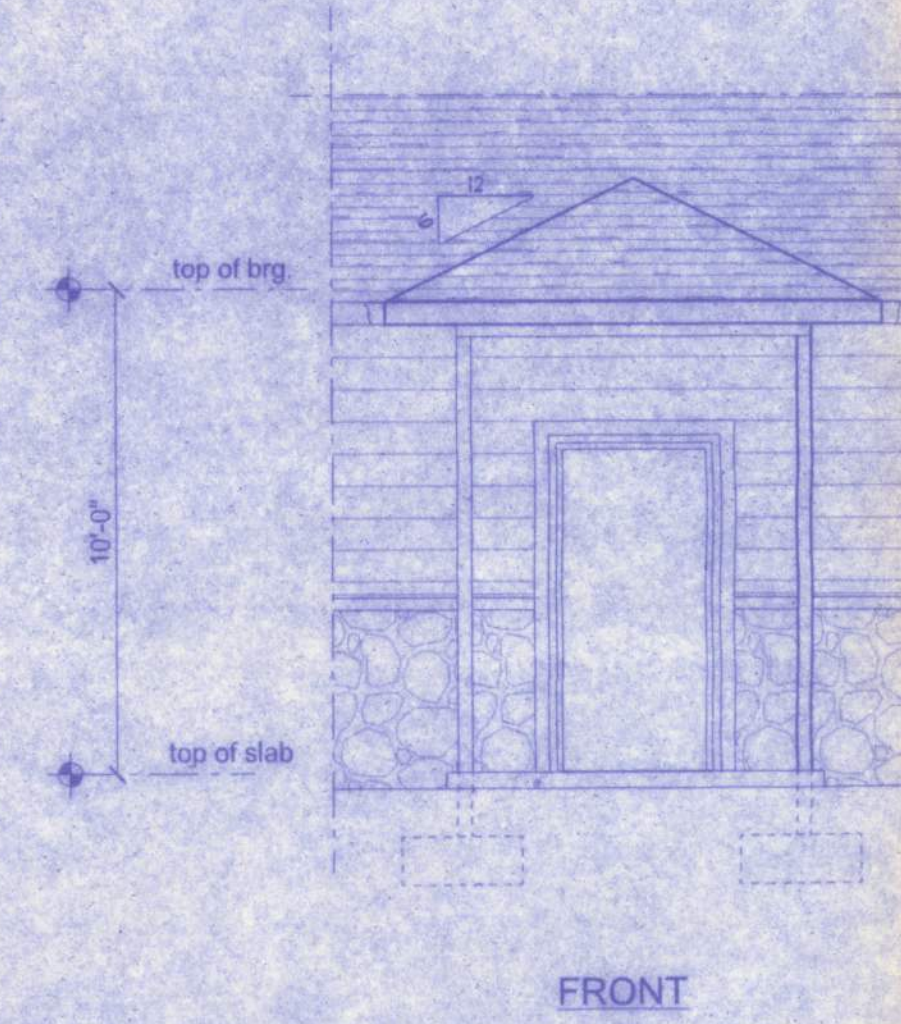
SOUTH ENTRANCE PORCH SCALE: 1/4" = 1'-0"
