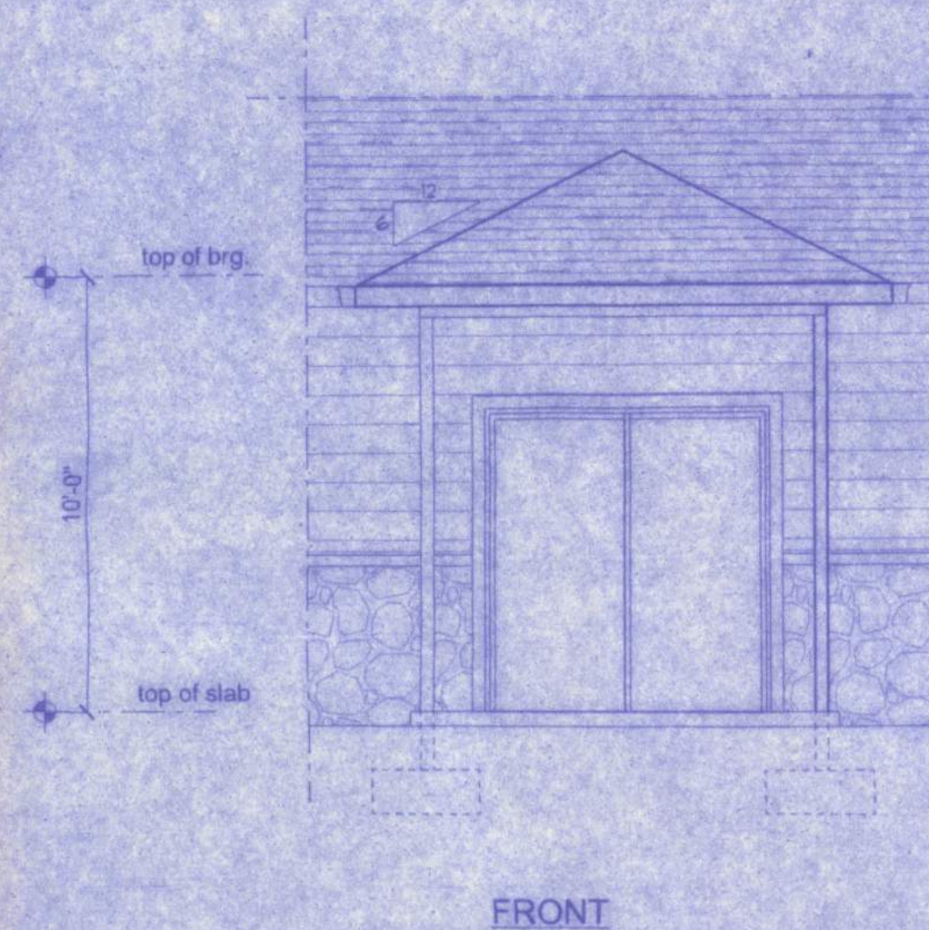
NORTH ENTRANCE PORCH SCALE: 1/4" = 1'-0"
