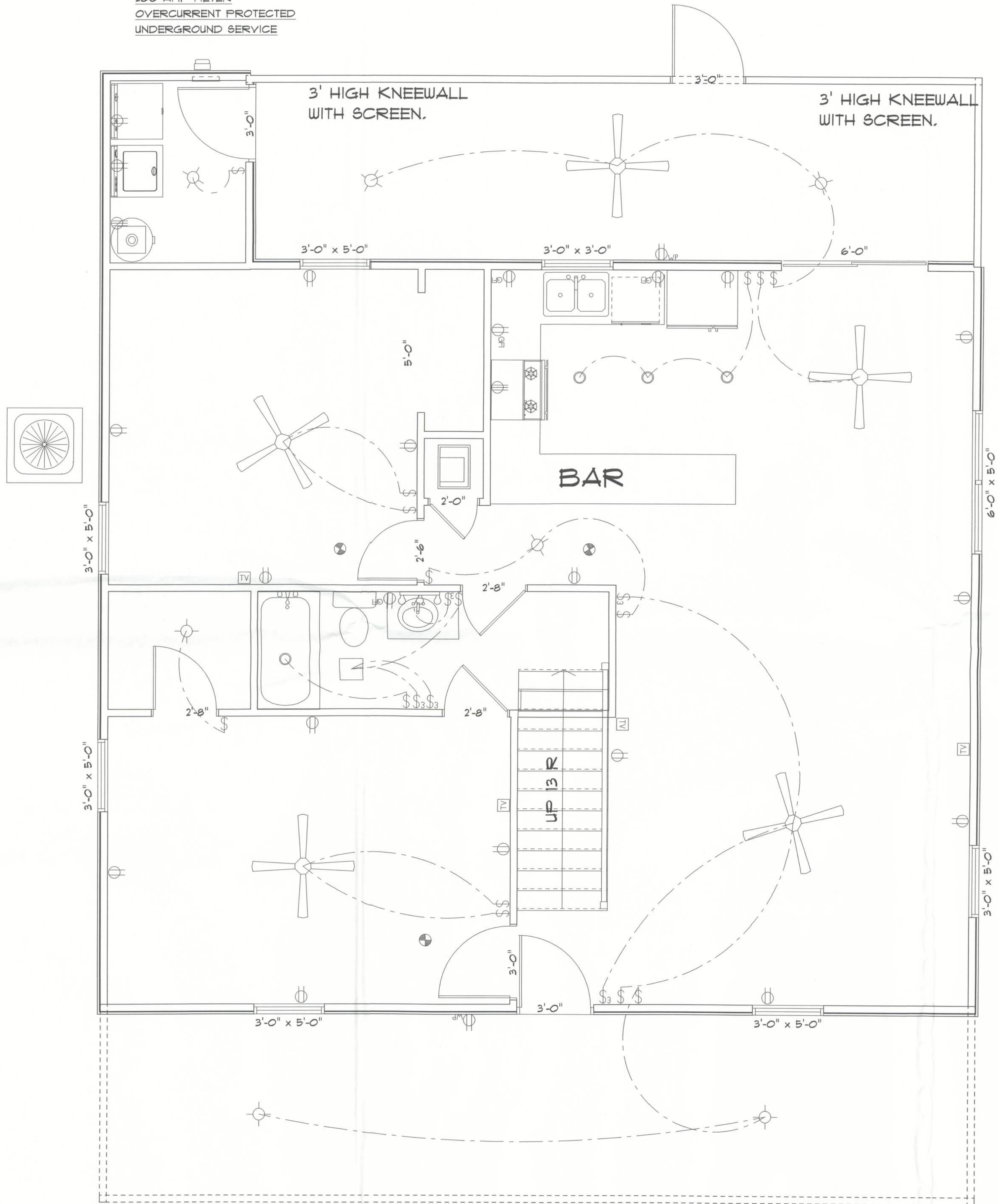
ELECTRICAL PLAN
