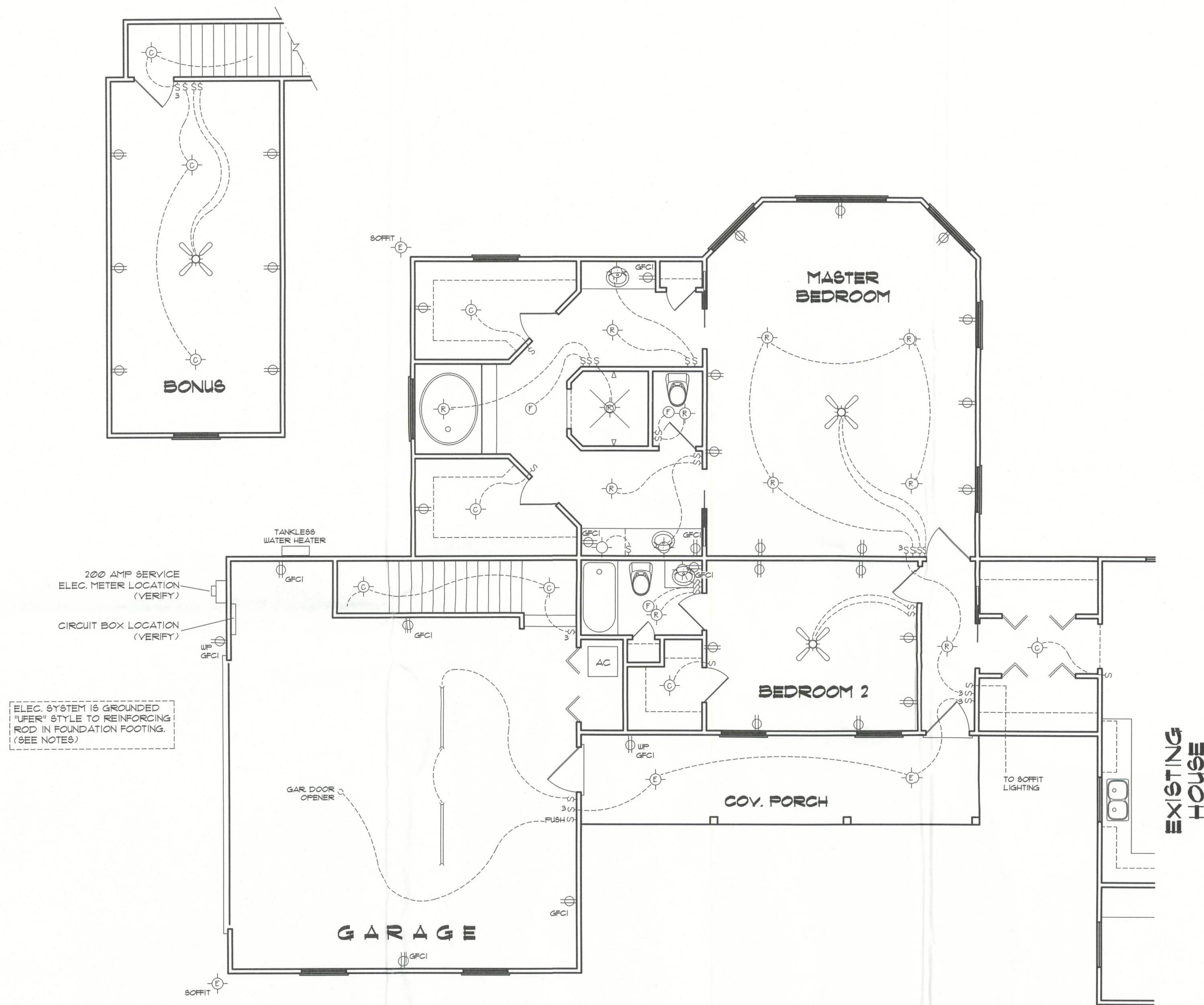
ELECTRICAL PLAN NOT TO SCALE
