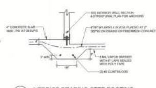
F4 INTERIOR BEARING STEP FOOTING SCALE: 1/2" = 1'-0"
