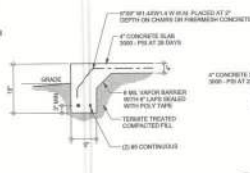
F2 MONOLITHIC FOOTING SCALE: 1/2" = 1'-0"
