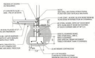
F1 STEM WALL FOOTING SCALE: 1/2" = 1'-0"
