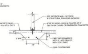
F3 INTERIOR BEARING FOOTING SCALE: 1/2" = 1'-0"
