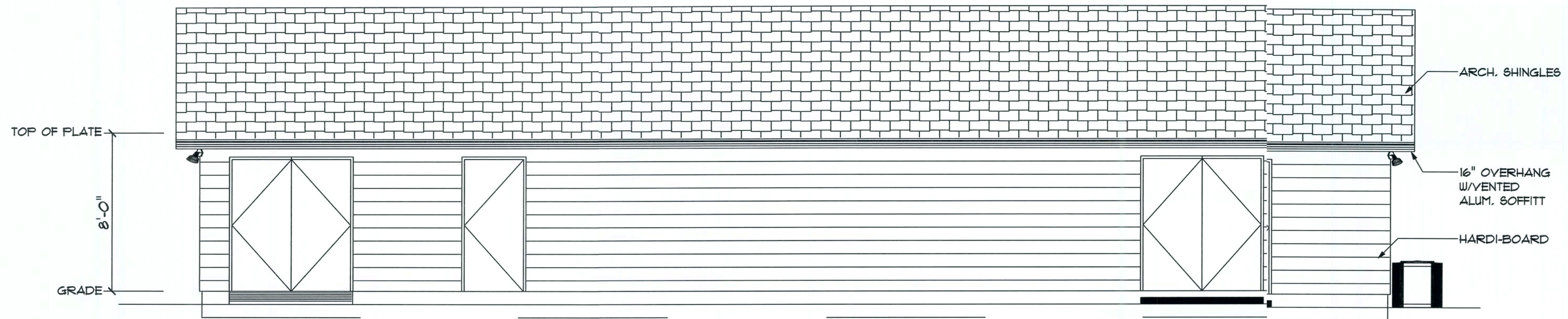
FRONT ELEVATION
