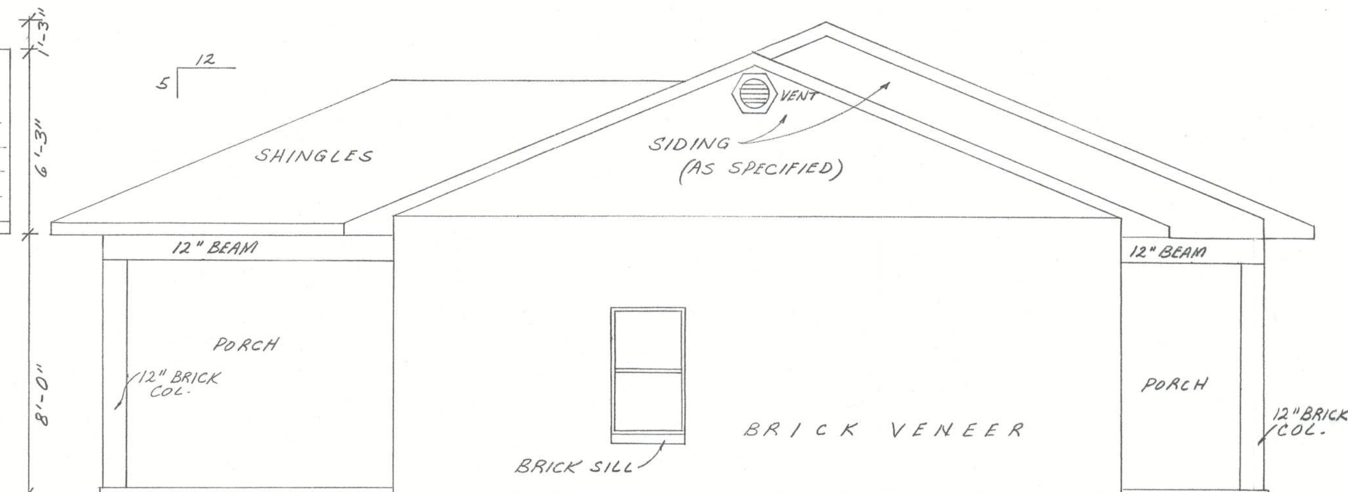
LEFT ELEVATION
