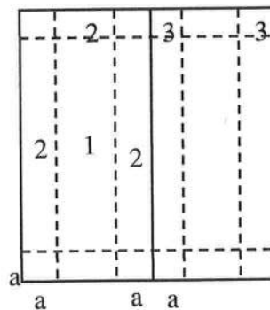
Figure 6-5 - External Pressure Coefficients, GCp
