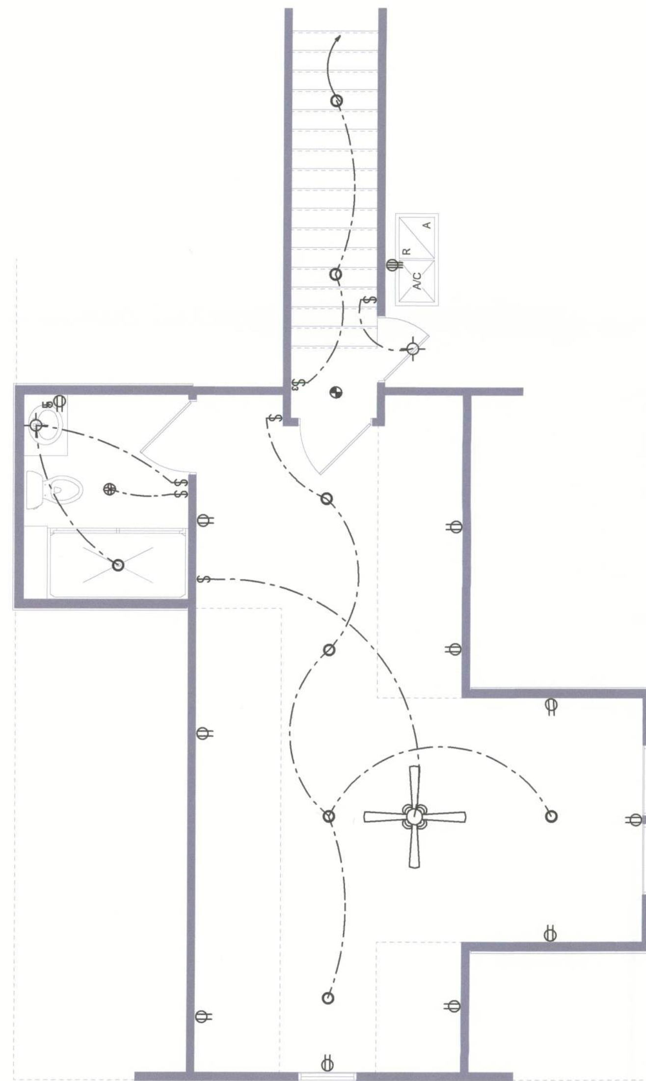
BONUS ROOM ELECTRICAL SCALE: 1/4" = 1'-0"
