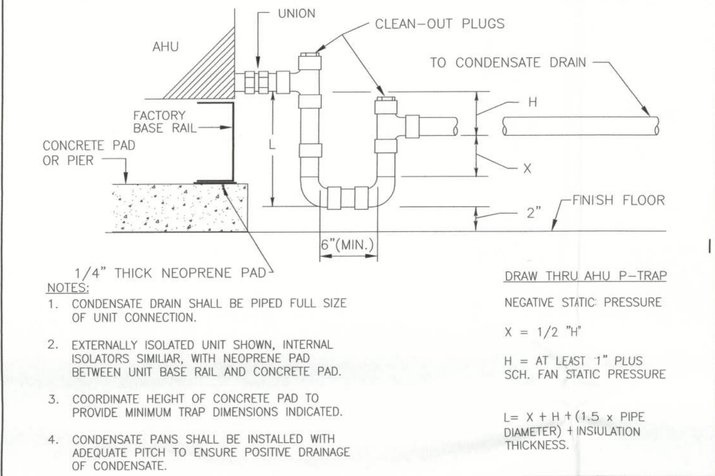
AHU CONDENSATE DRAIN DETAIL NTS DET 5 M3
