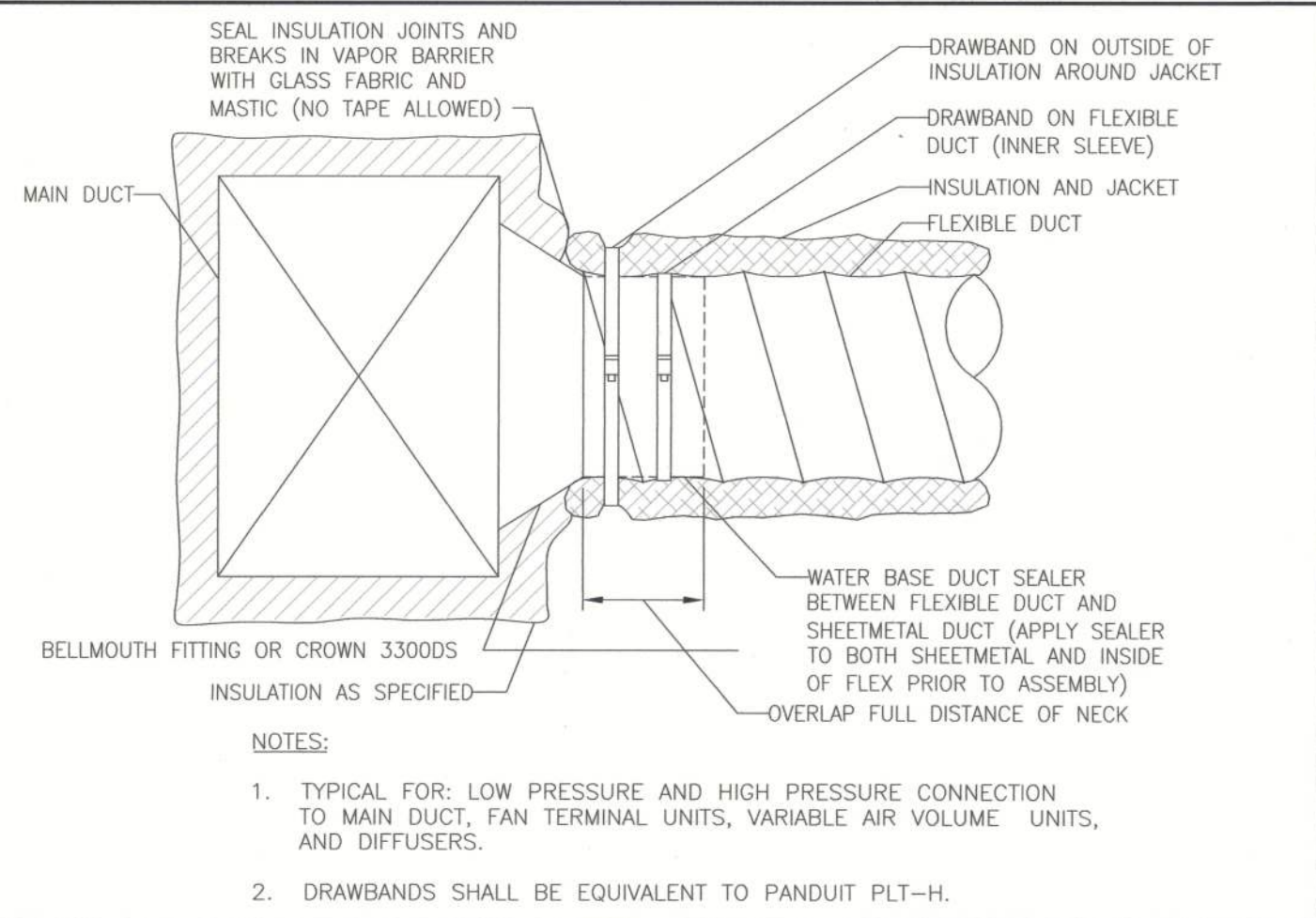
FLEXIBLE DUCT TAKEOFF DETAIL DET 2 M3
