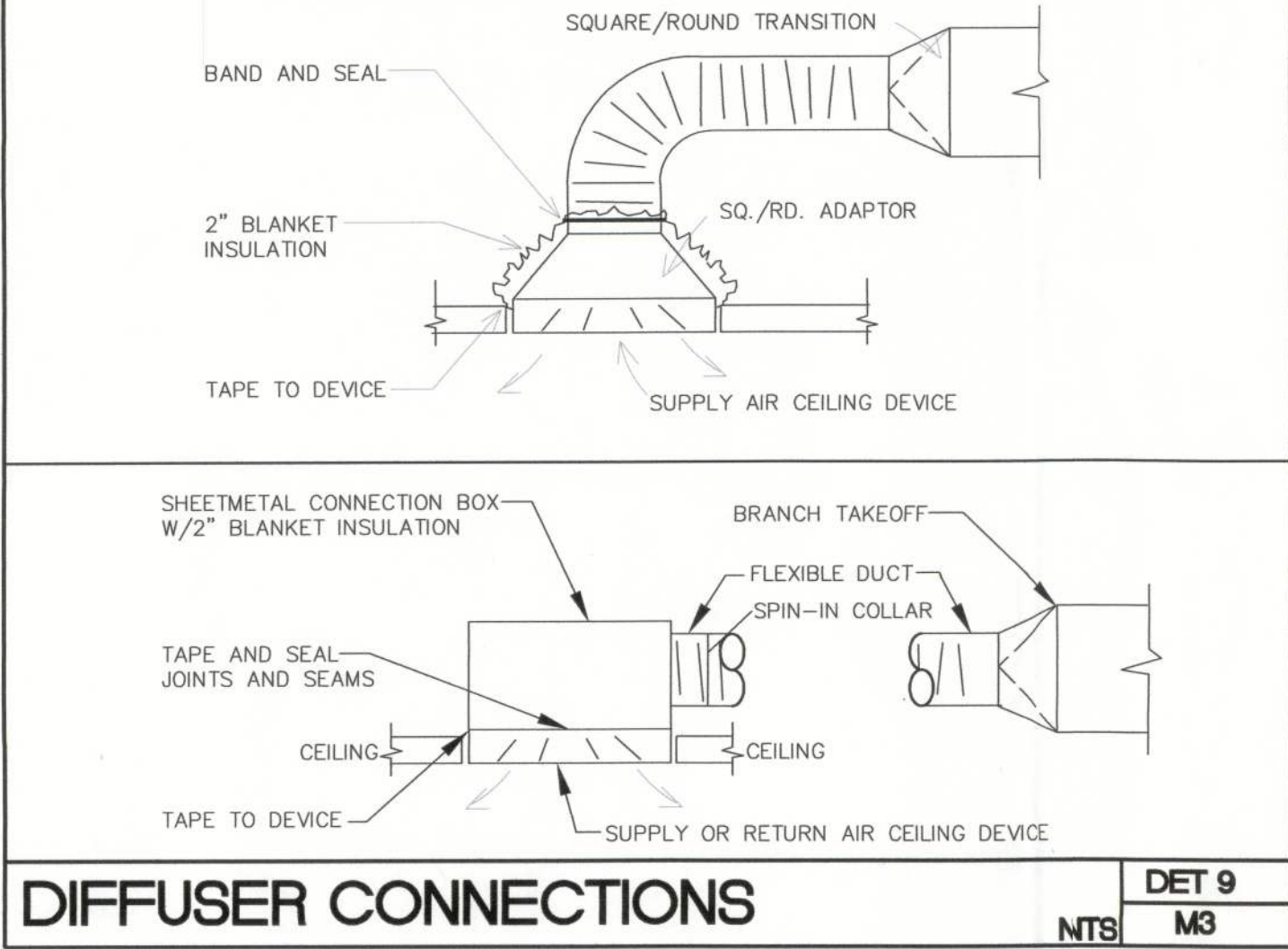
DIFFUSER CONNECTIONS NTS DET 9 M3
