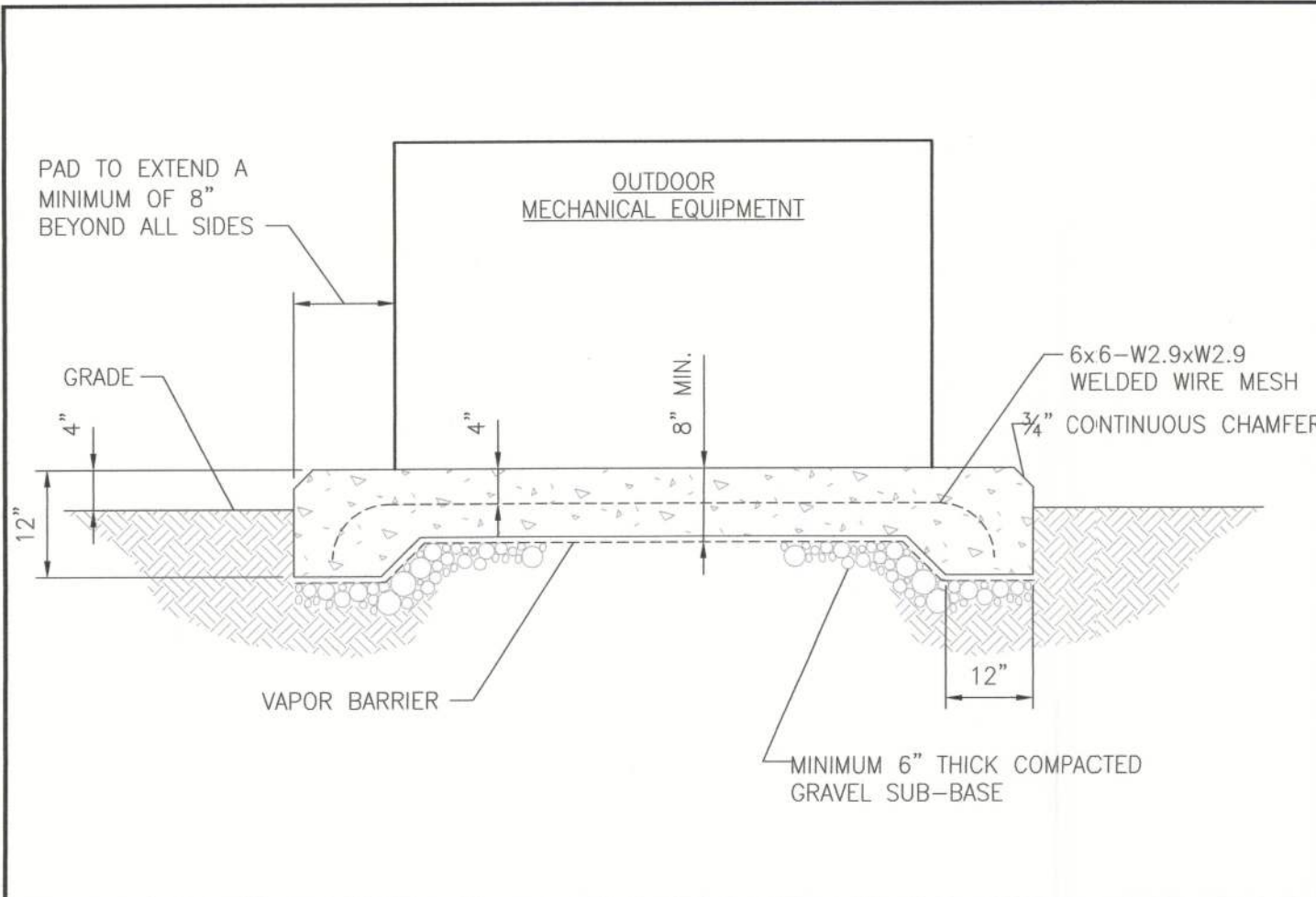
EQUIPMENT PAD DETAIL NTS DET 1 M3
