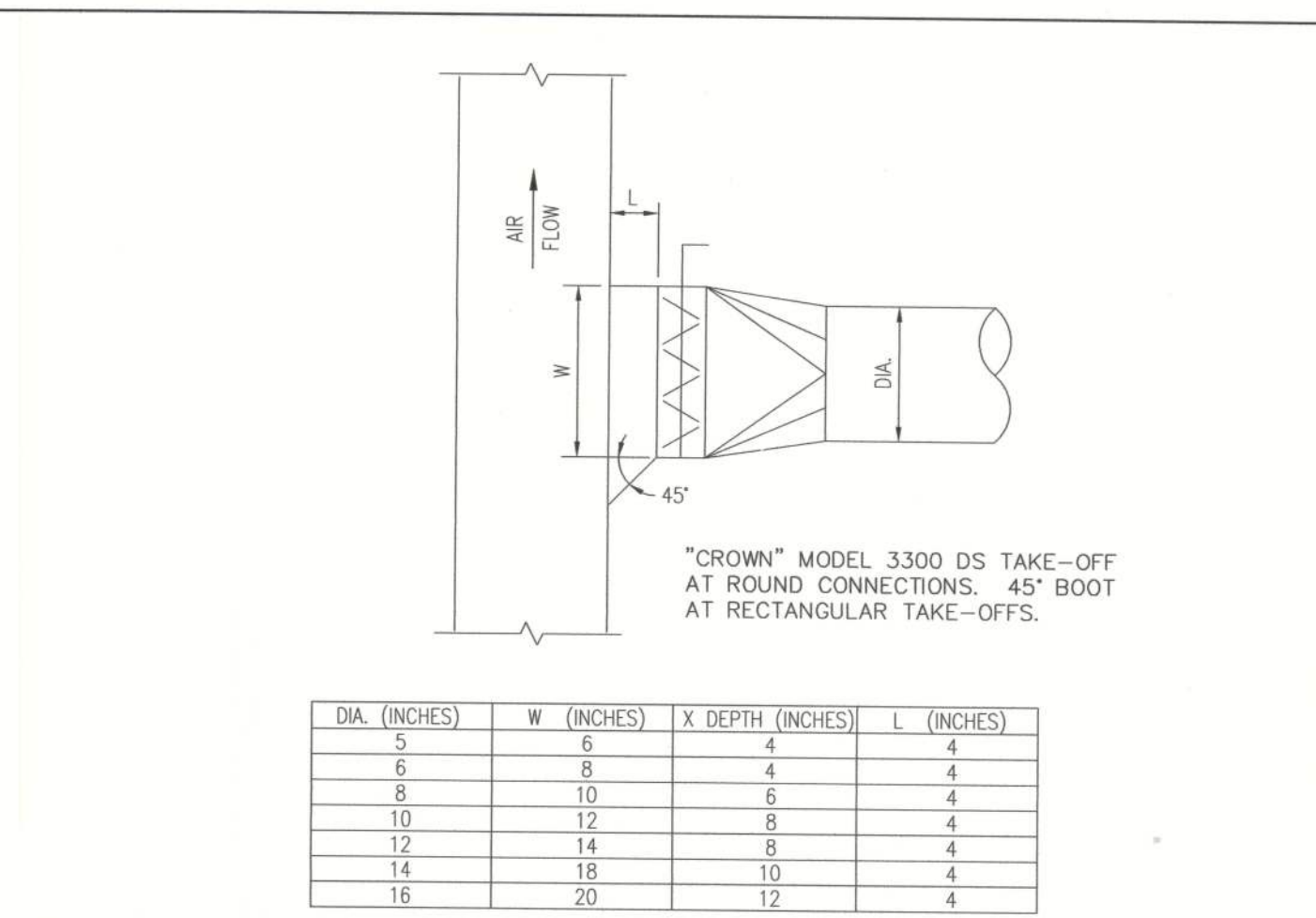
ROUND DUCT TAKEOFF DETAIL DET 4 M3
