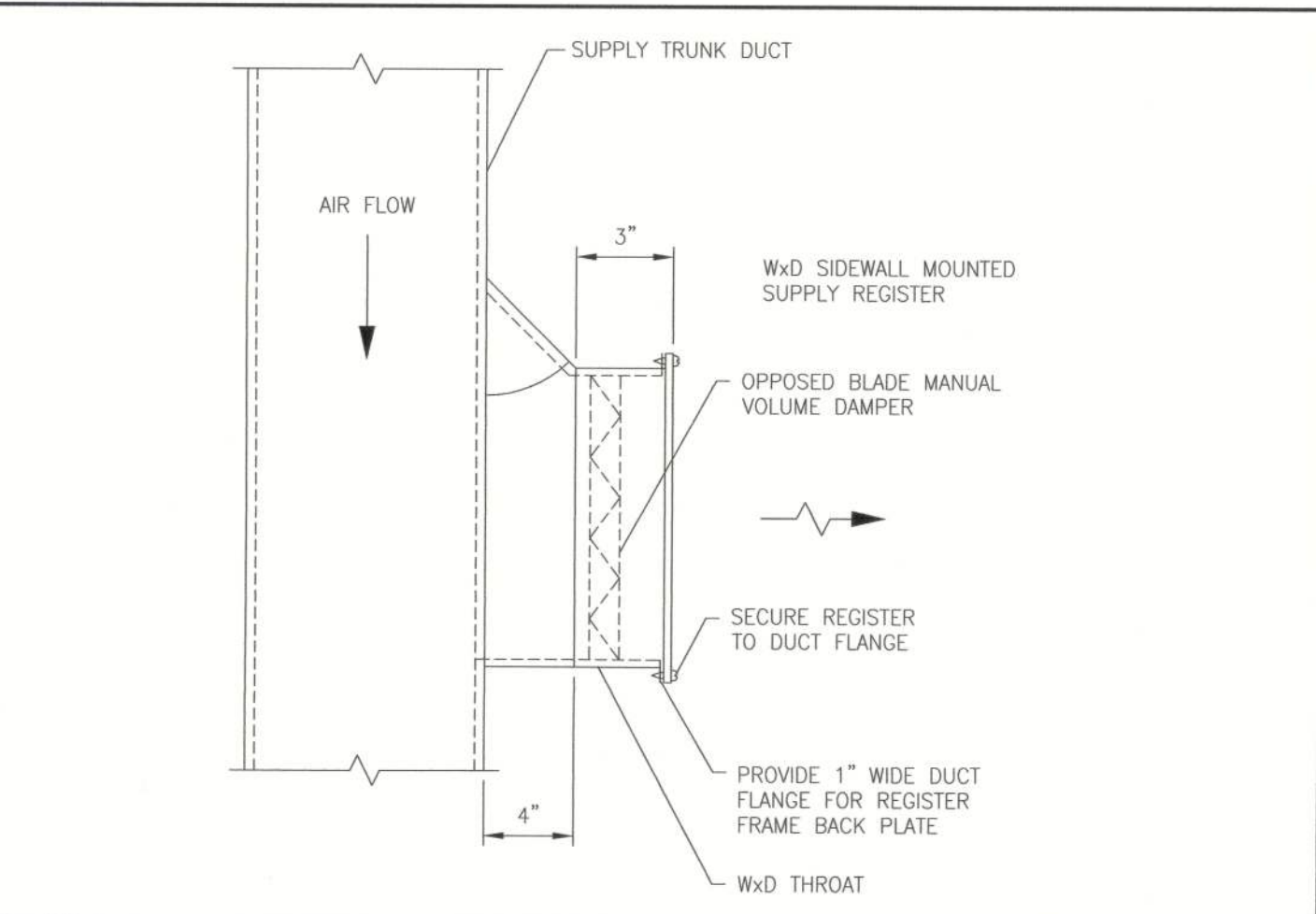
RECTANGULAR DUCT TAKEOFF DETAIL DET 3 M3
