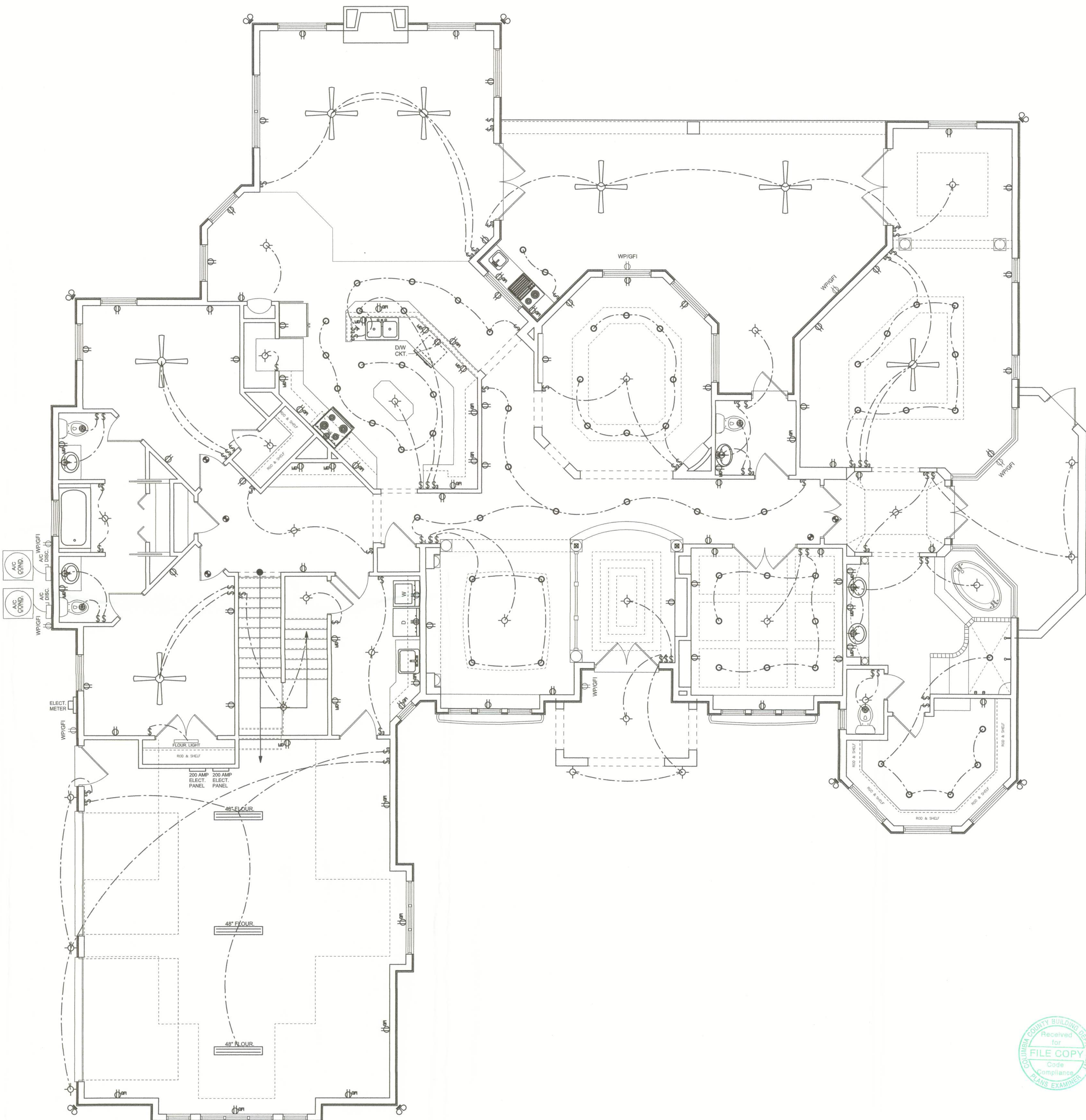
ELECTRICAL PLAN SCALE: 1/4" = 1'-0"
