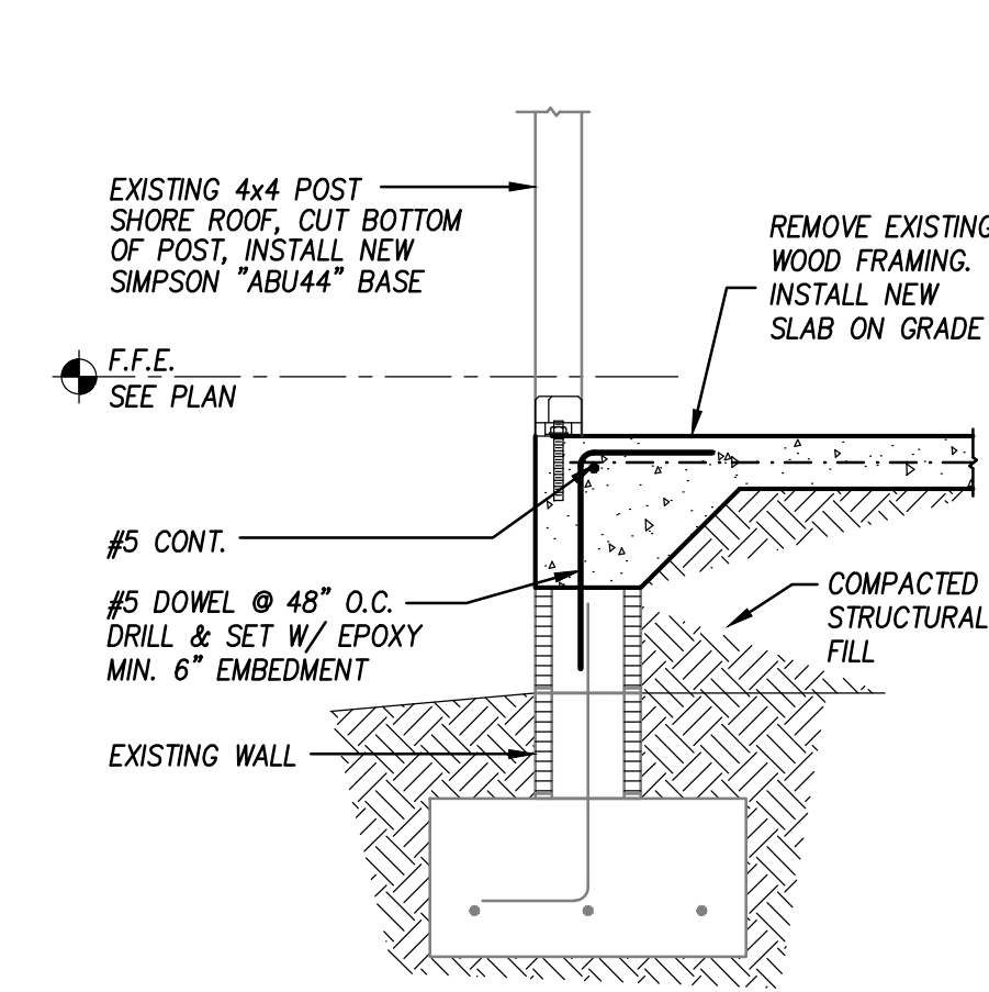
F19 Foundation Section 3/4" = 1'-0" MAS-W402
