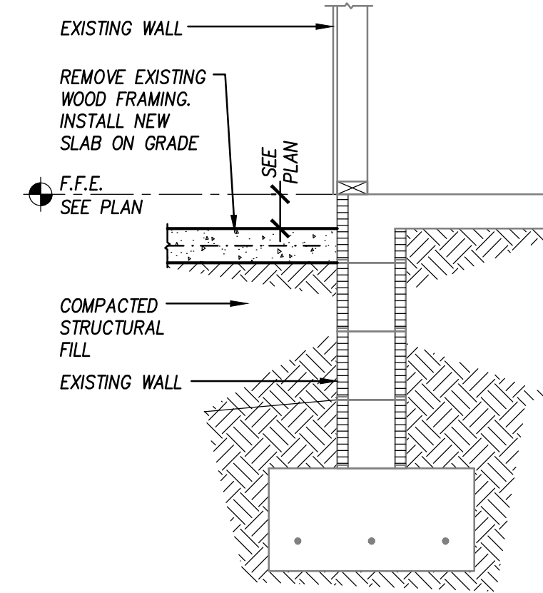
F21 Foundation Section 3/4" = 1'-0" MAS-W404
