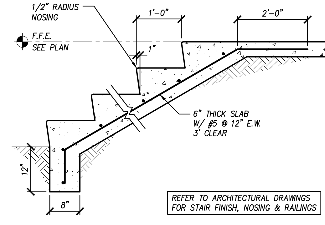
F16 Typical Stair Section 3/4" = 1'-0" STAIR-001
