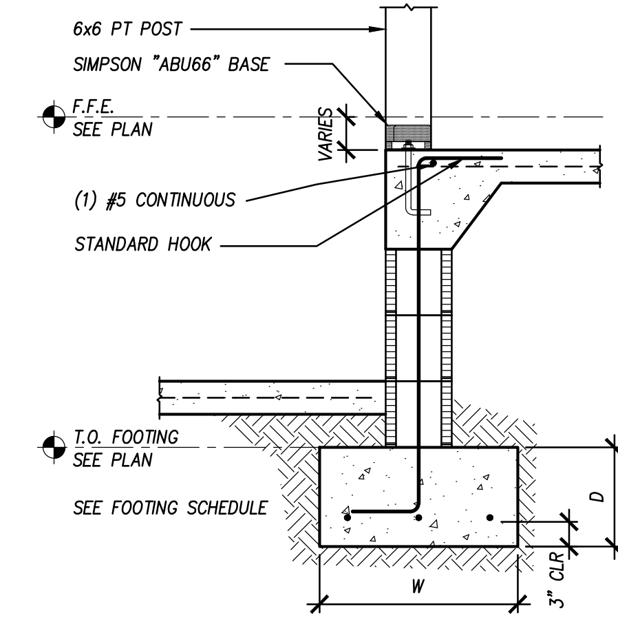
F15 Foundation Section 3/4" = 1'-0" MAS-W505
