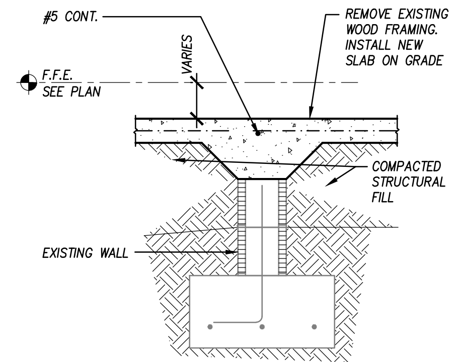
F20 Foundation Section 3/4" = 1'-0" MAS-W403
