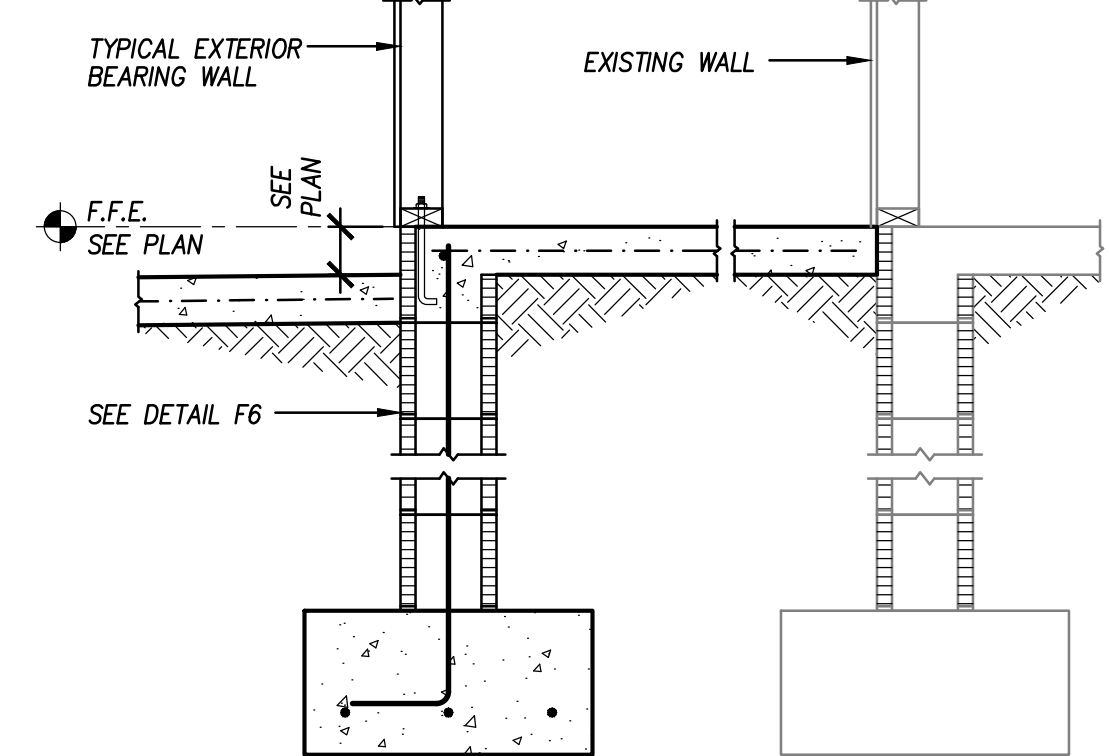
F22 Foundation Section 3/4" = 1'-0" MAS-W405
