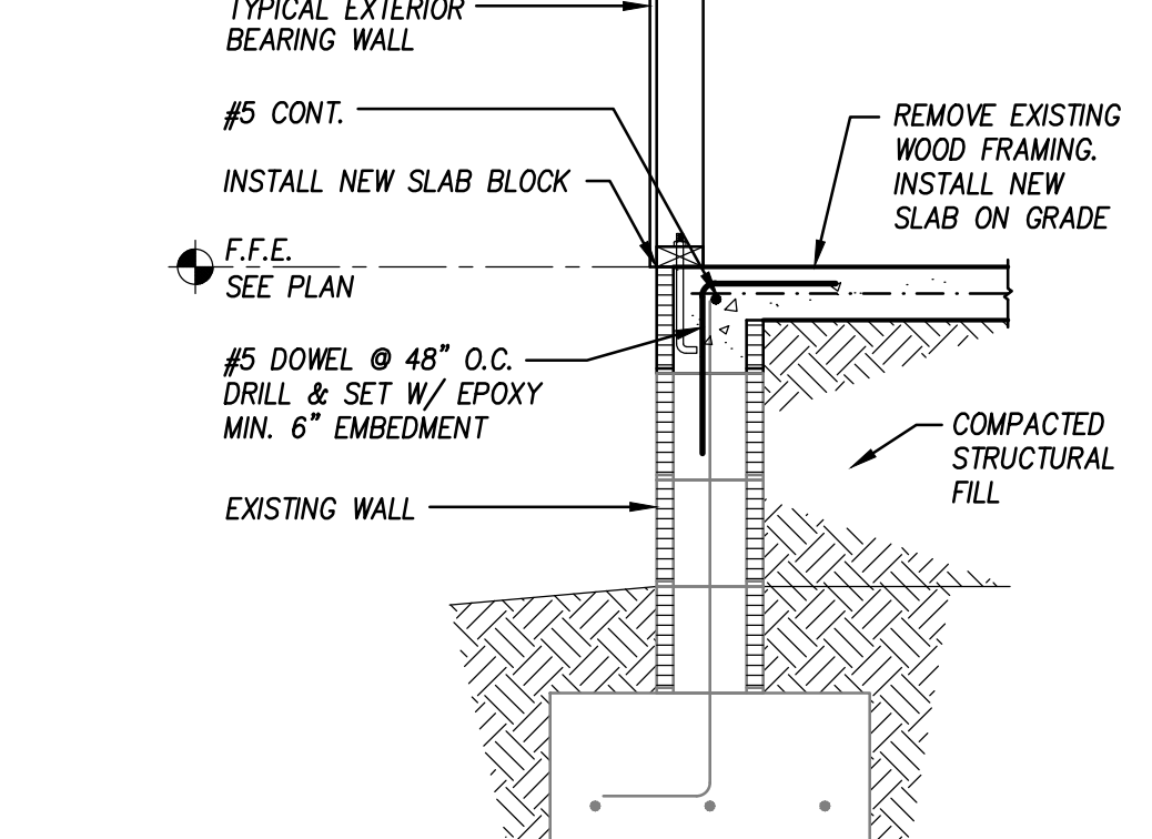
F18 Foundation Section 3/4" = 1'-0" MAS-W401
