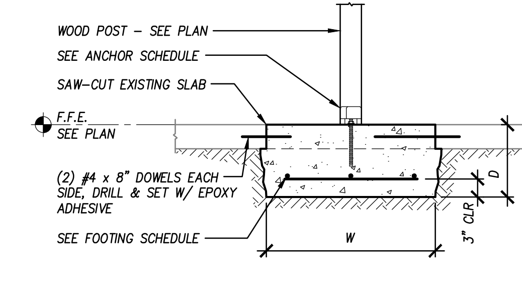
F17 Typical Footing Section 3/4" = 1'-0" MONO120
