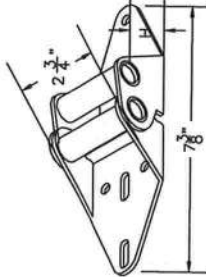
P/N 20604 (#1 HINGE)
