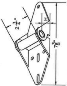
P/N 20604 (#1 HINGE)
