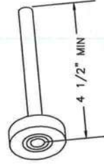
P/N 20812 SHORT STEM 11 BALL NYLON COATED STEEL ROLLER
