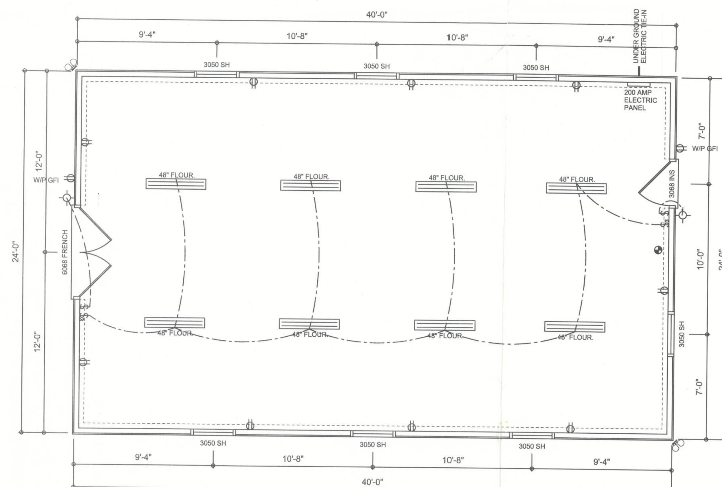
DIMENSIONED FLOOR PLAN SCALE: 1/4" = 1'-0"
