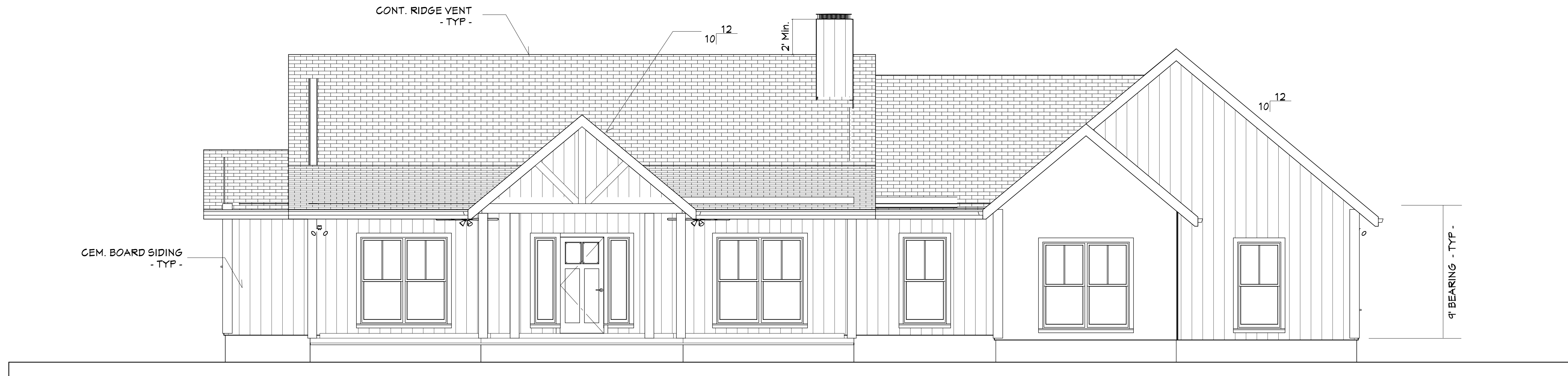
Front Elevation
