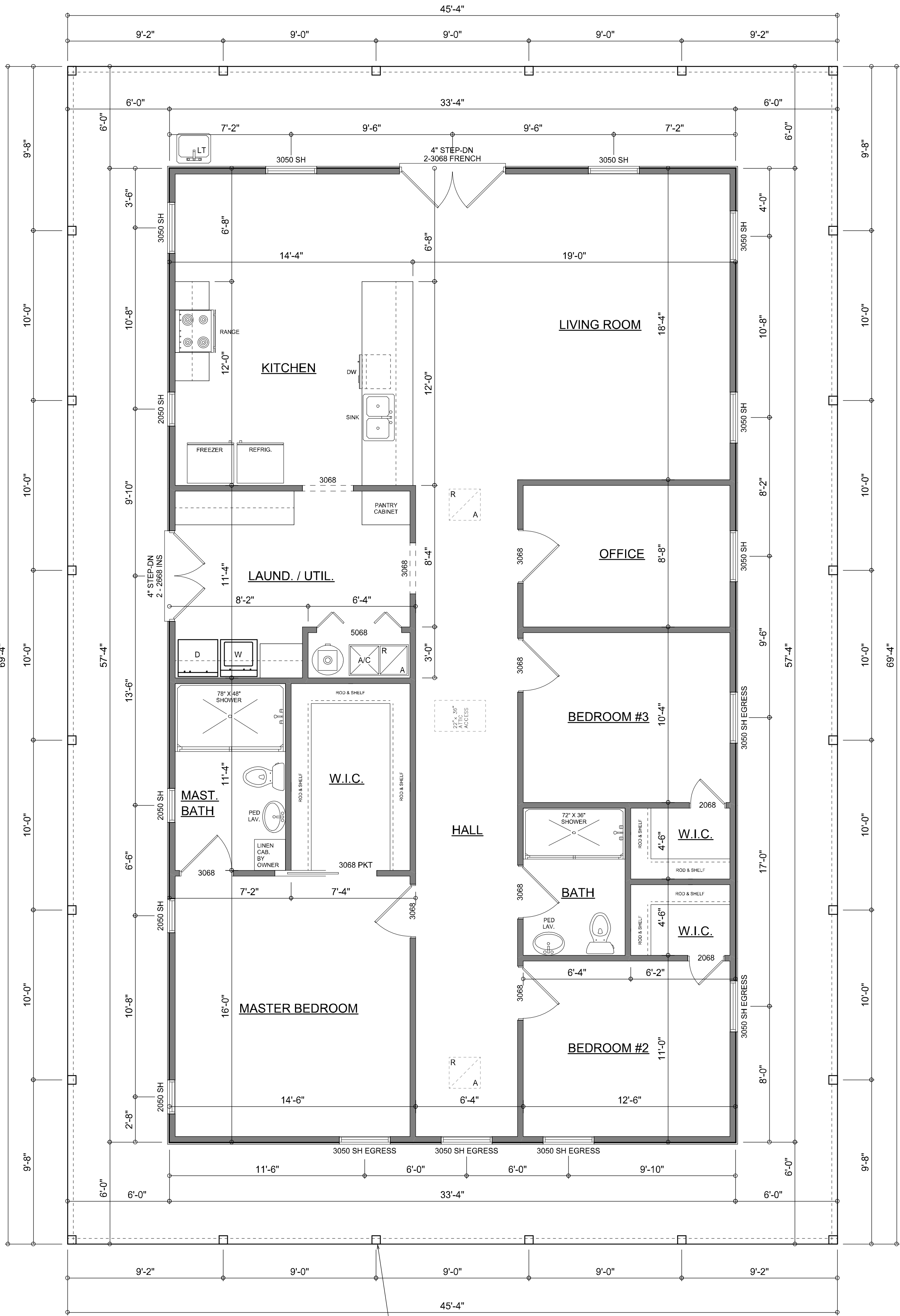
DIMENSIONED FLOOR PLAN SCALE: 1/4" = 1'-0"
