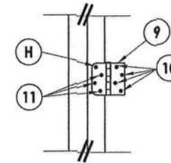
HINGE DETAIL
