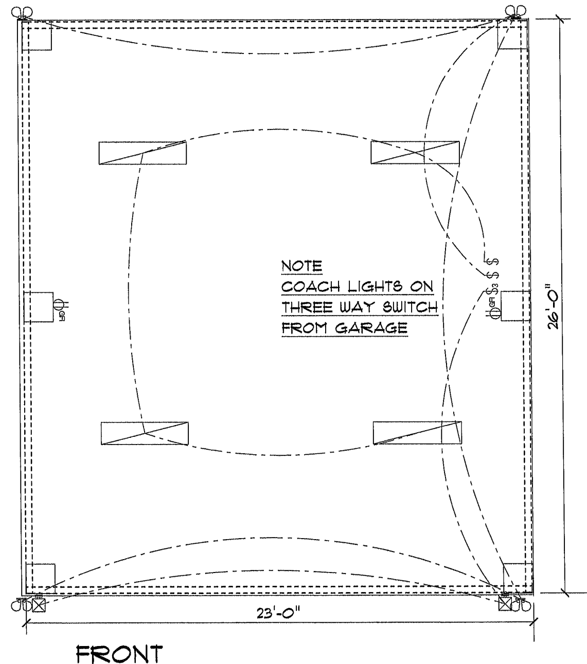
ELECTRICAL PLAN
