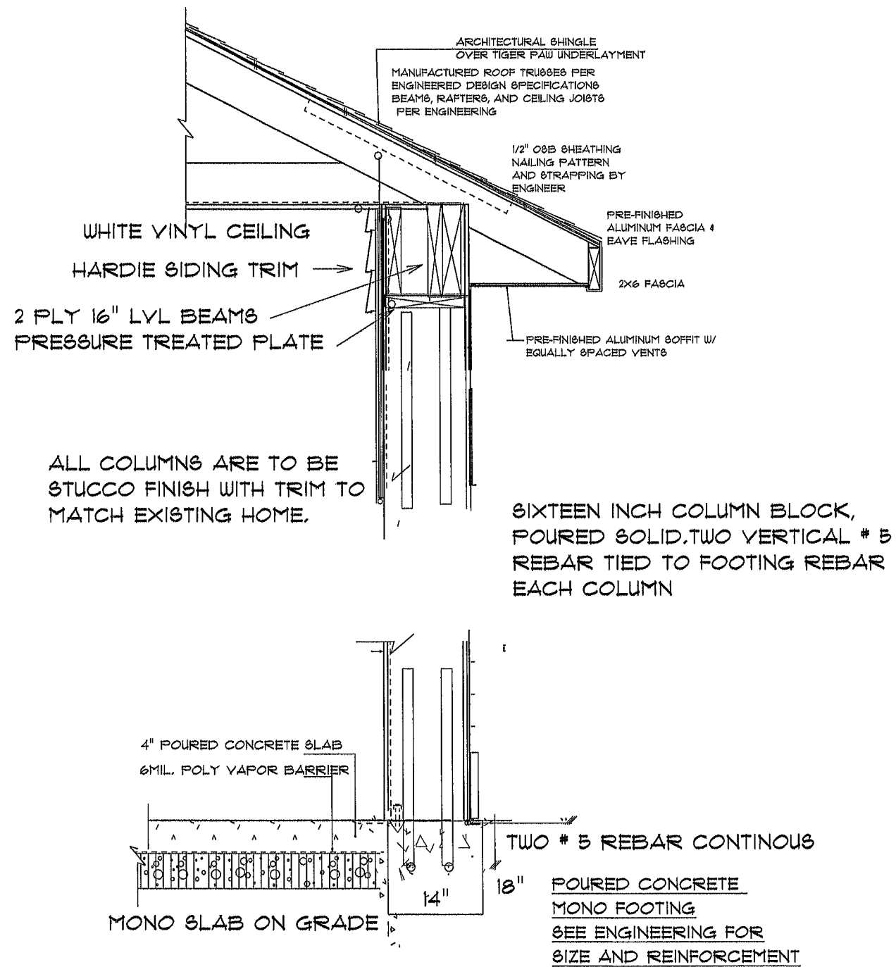
TYPICAL WALL SECTION NON - STRUCTURAL DATA
