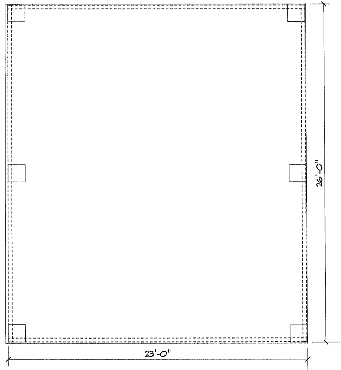
FLOOR PLAN
