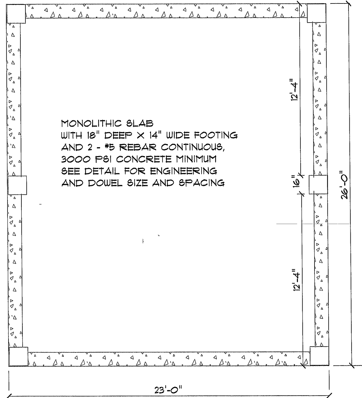
FOUNDATION / MONOLITHIC SLAB
