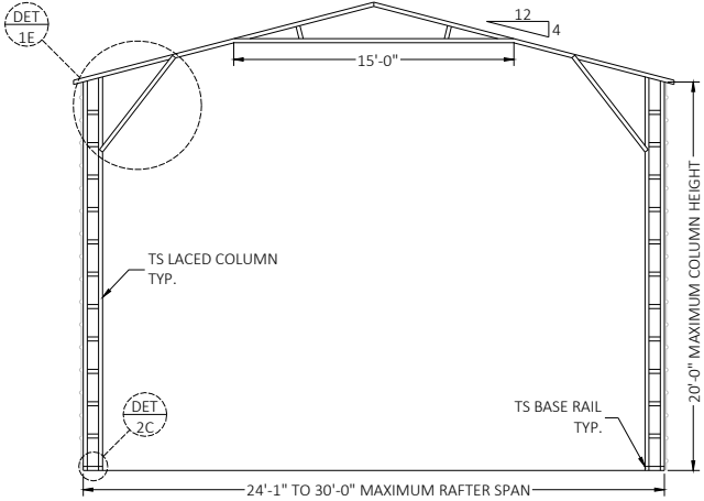
BOX EAVE FRAME
