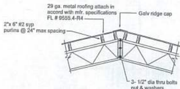
RIDGE CONNECTION DETAIL
