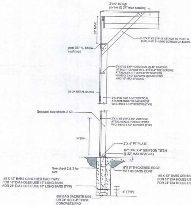
POST FOOTING TO TRUSS DETAIL SECTION 1
