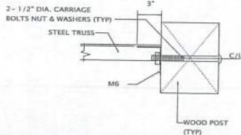
TRUSS TO POST DETAIL PLAN VIEW
