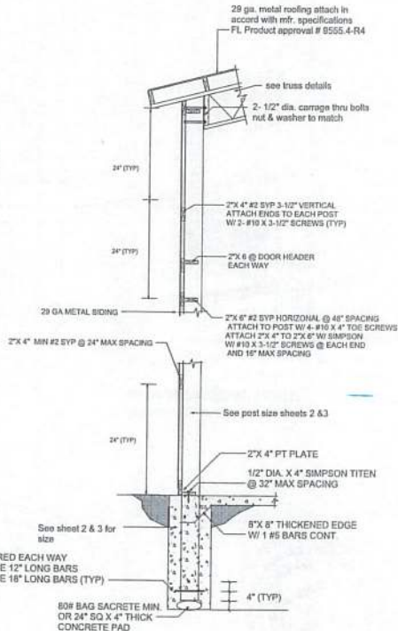
POST FOOTING TO TRUSS DETAIL SECTION 2
