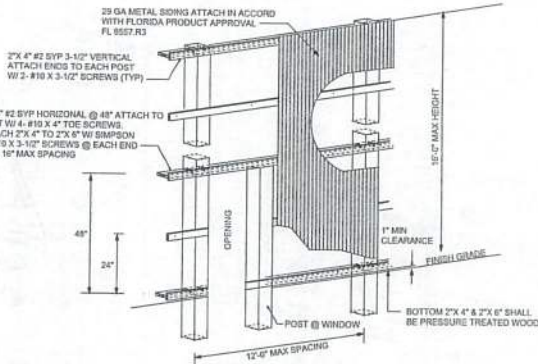
150 MPH SOLID WALL DESIGN
