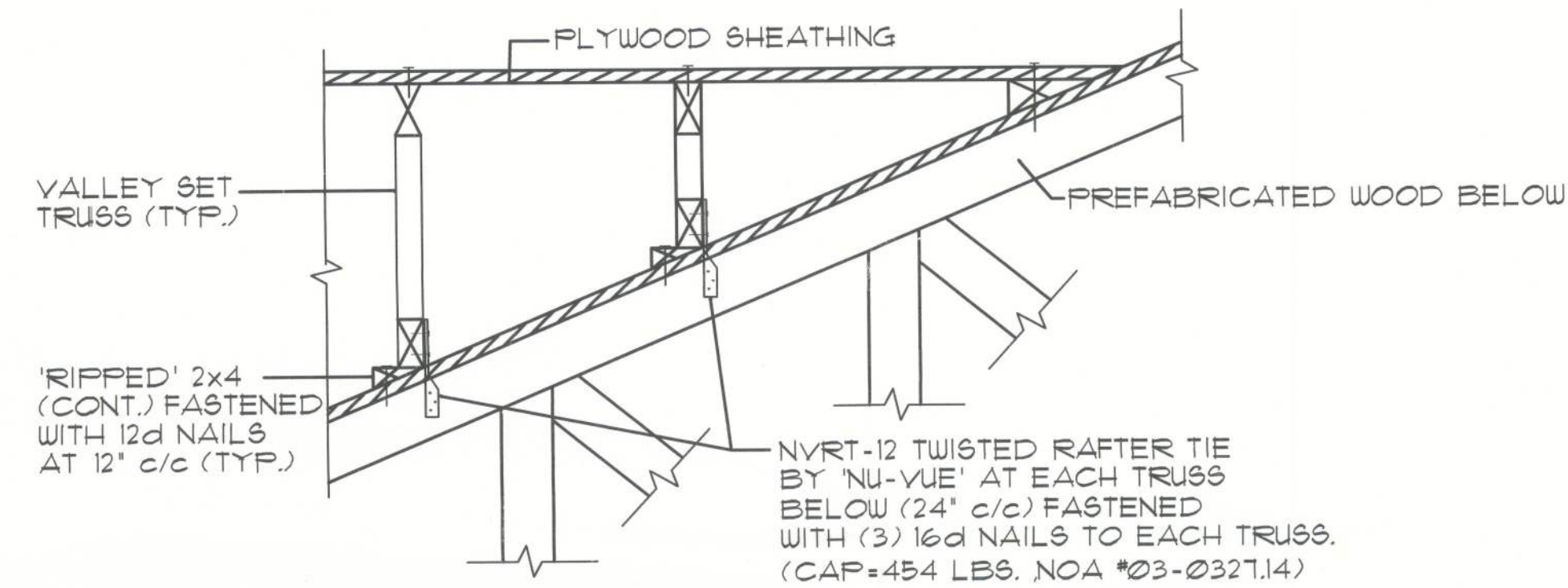
B TYPICAL VALLEY SET ("PIGGYBACK") TRUSS TIE-DOWN DETAIL
