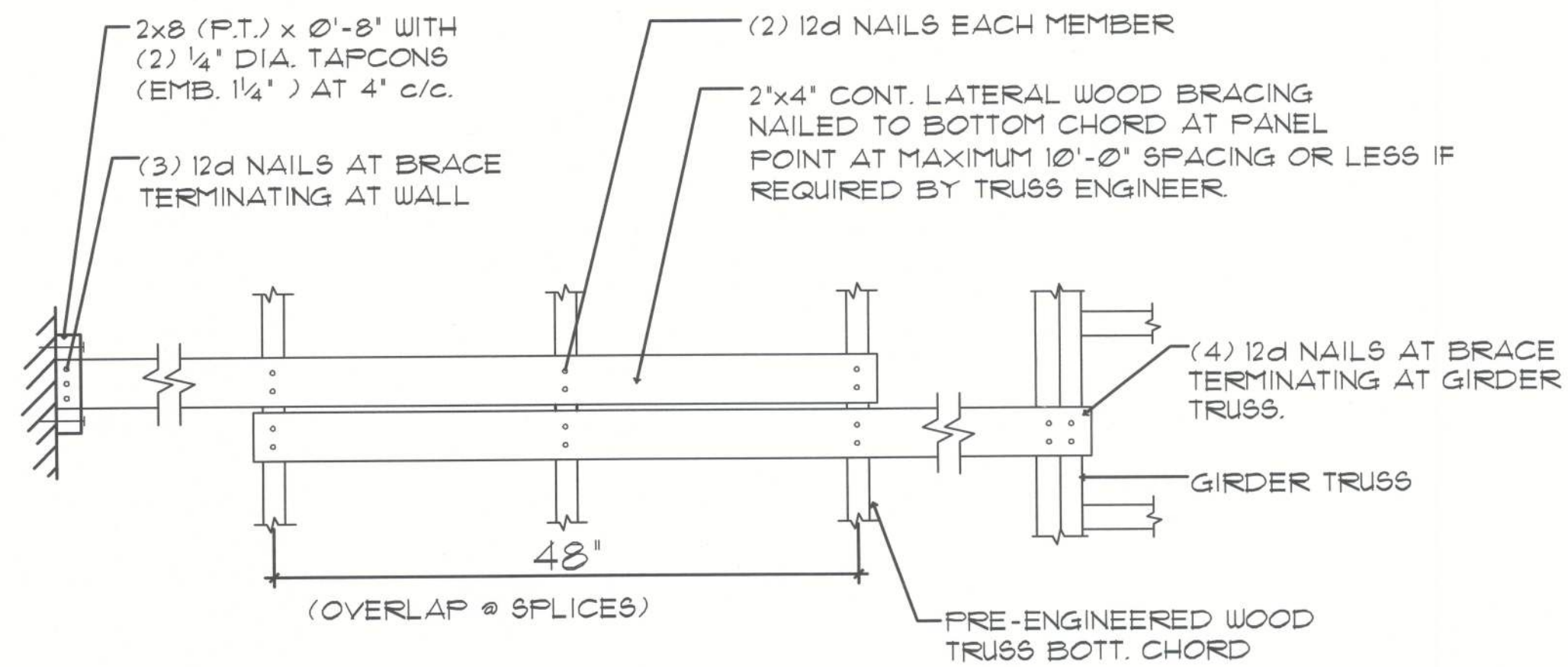
B CONTINUOUS LATERAL TRUSS BRACING DETAIL
