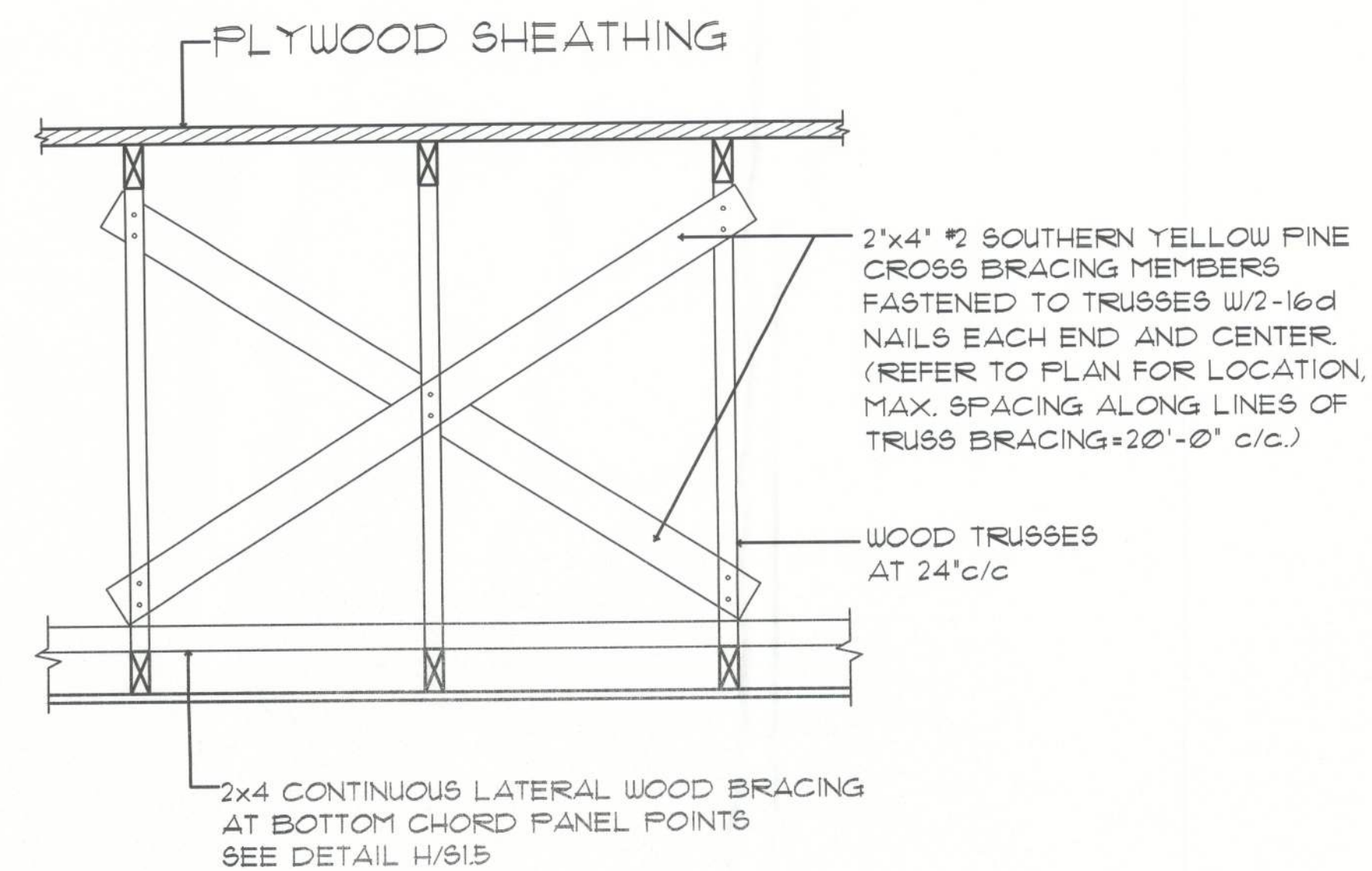
B TYPICAL TRUSS X-BRACING DETAIL
