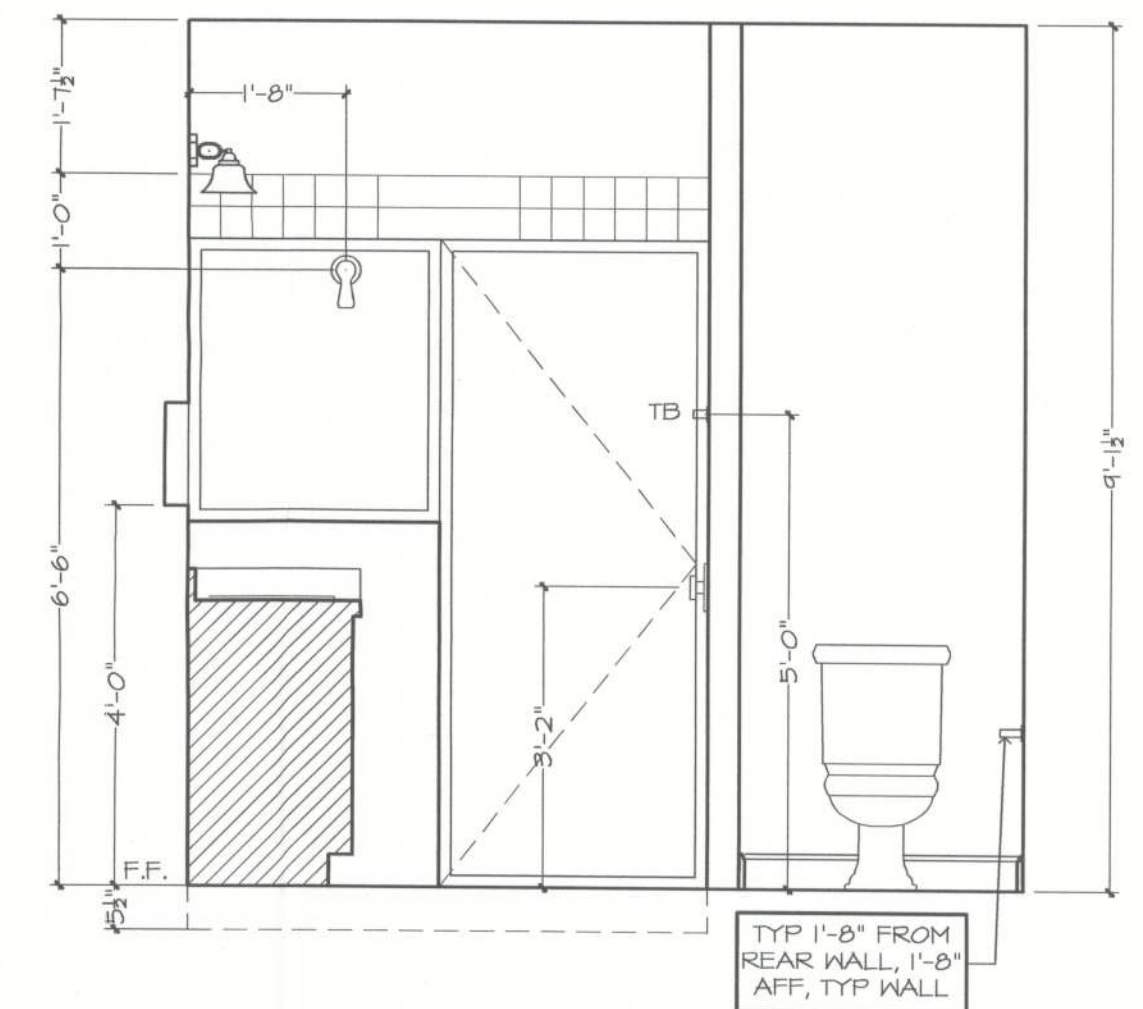
WALL "Z"
