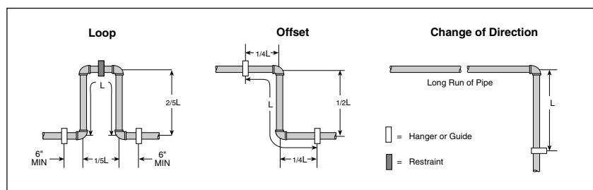
Figure G • Expansion Loop and Offset Configurations
