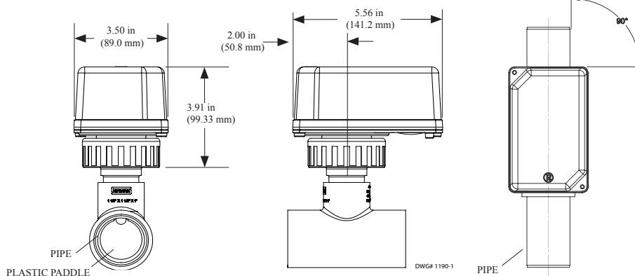
Fig. 7 Mounting Dimensions-Orientation
