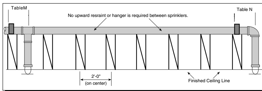
Wood Frame Construction
