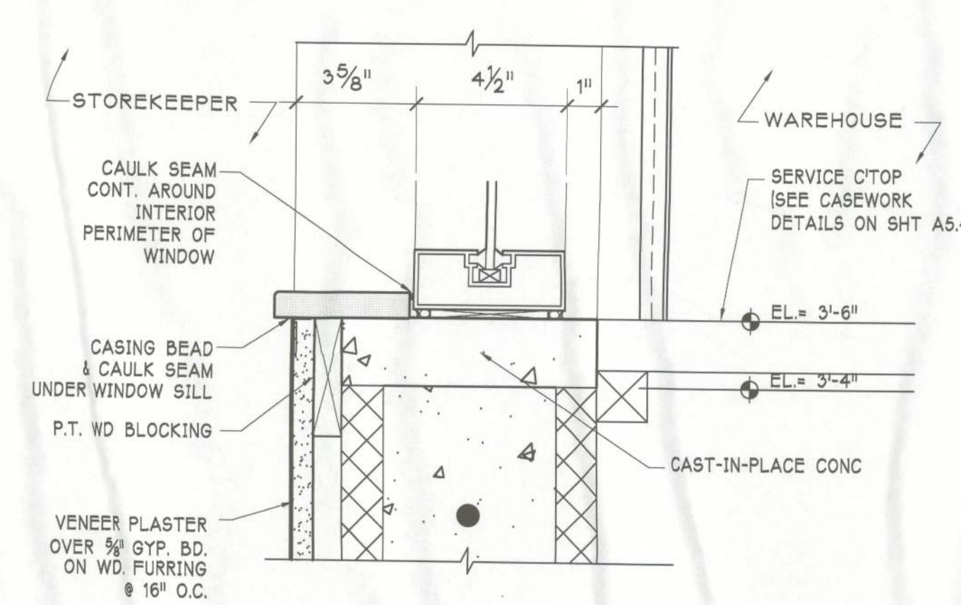
SILL / COUNTER FIRE SHUTTER SCALE: 3" = 1'-0"
