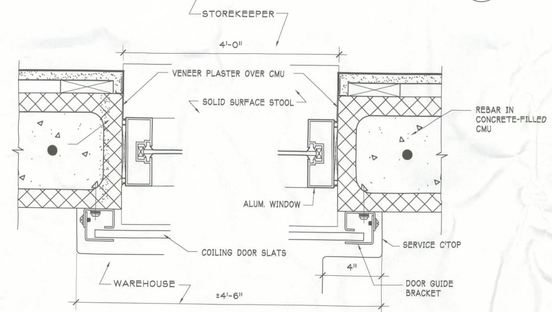
JAMB / COUNTER FIRE SHUTTER SCALE: 3" = 1'-0"
