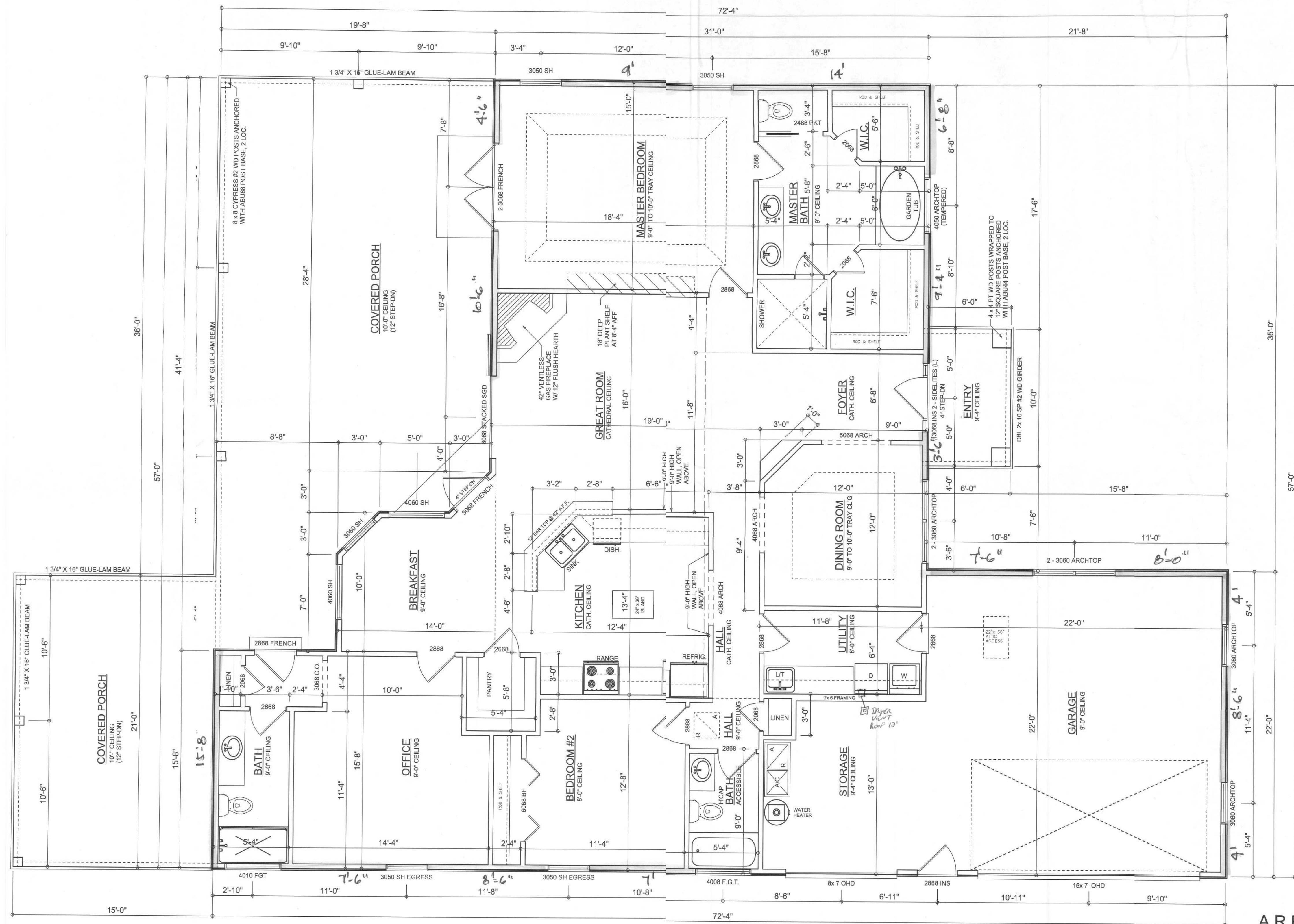
FLOOR PLAN SCALE: 1/4" = 1'-0" NOTE: ALL CEILINGS SHALL BE 9'-0" UNLESS OTHERWISE NOTED.
