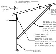
1.1 BOX EAVE RAFTER COLUMN CONNECTION DETAIL FOR HEIGHTS 12'-0" < H <= 15'-0" SCALE: NTS
