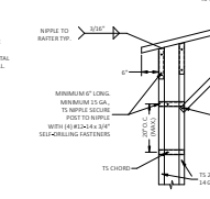
1B BOX EAVE RAFTER COLUMN CONNECTION DETAIL FOR HEIGHTS 16'-0" < H <= 18'-0" SCALE: NTS
