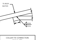
COLLAR TIE CONNECTION SCALE: NTS
