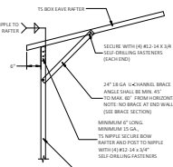
1.2 BOX EAVE RAFTER COLUMN CONNECTION DETAIL FOR HEIGHTS 12'-0" < H <= 15'-0" SCALE: NTS
