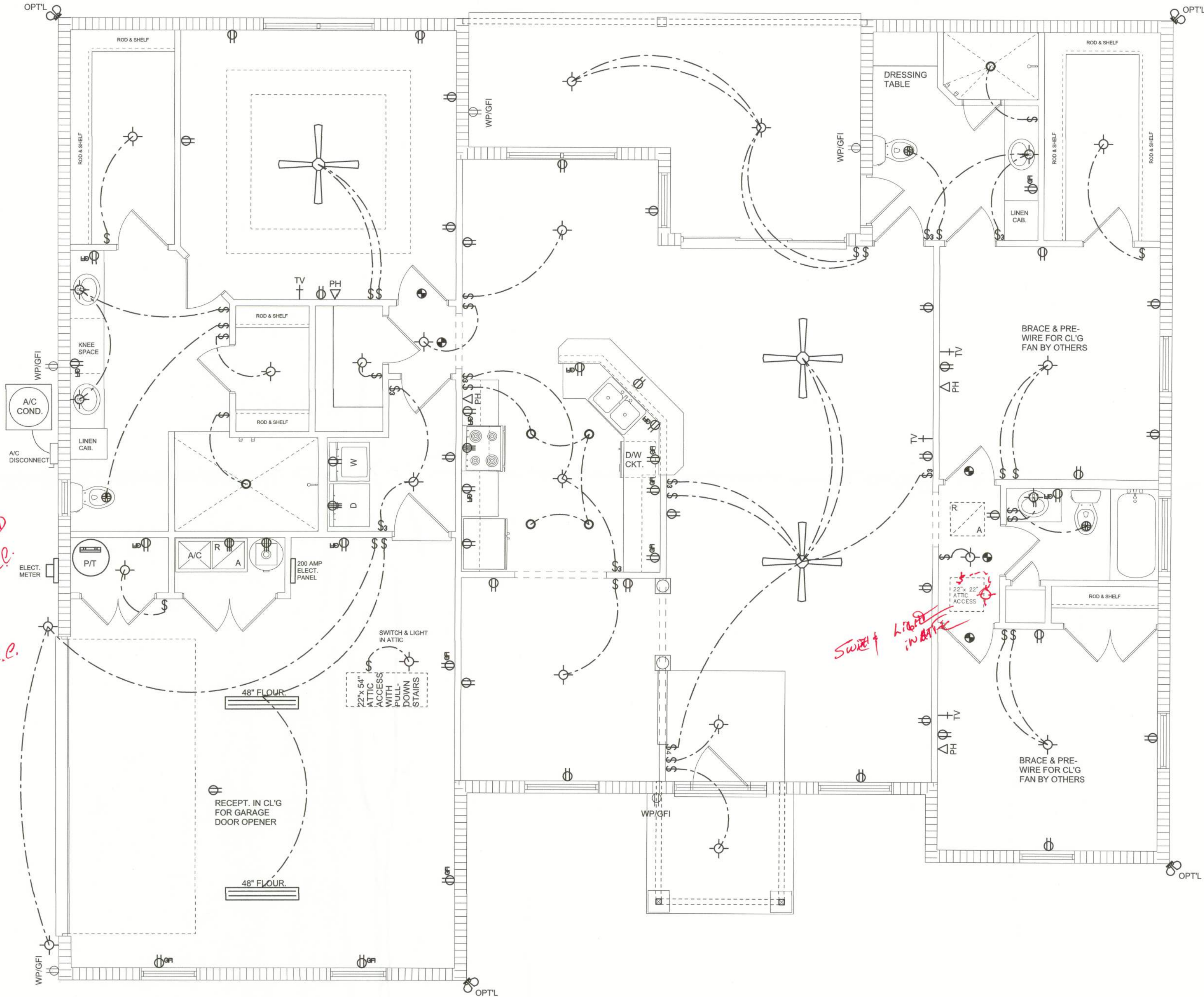
ELECTRICAL PLAN SCALE: 1/4\"/>
