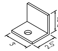
OPTION A L 2 1/2" X 2 1/2" X 3/16"
