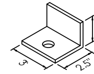
OPTION B L 2 1/2" X 2" X 3/16" SLV
