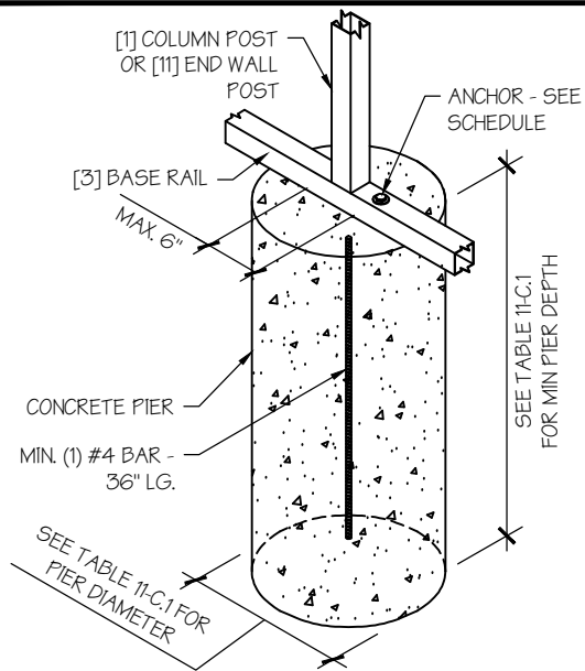
CONCRETE PIER DETAIL
