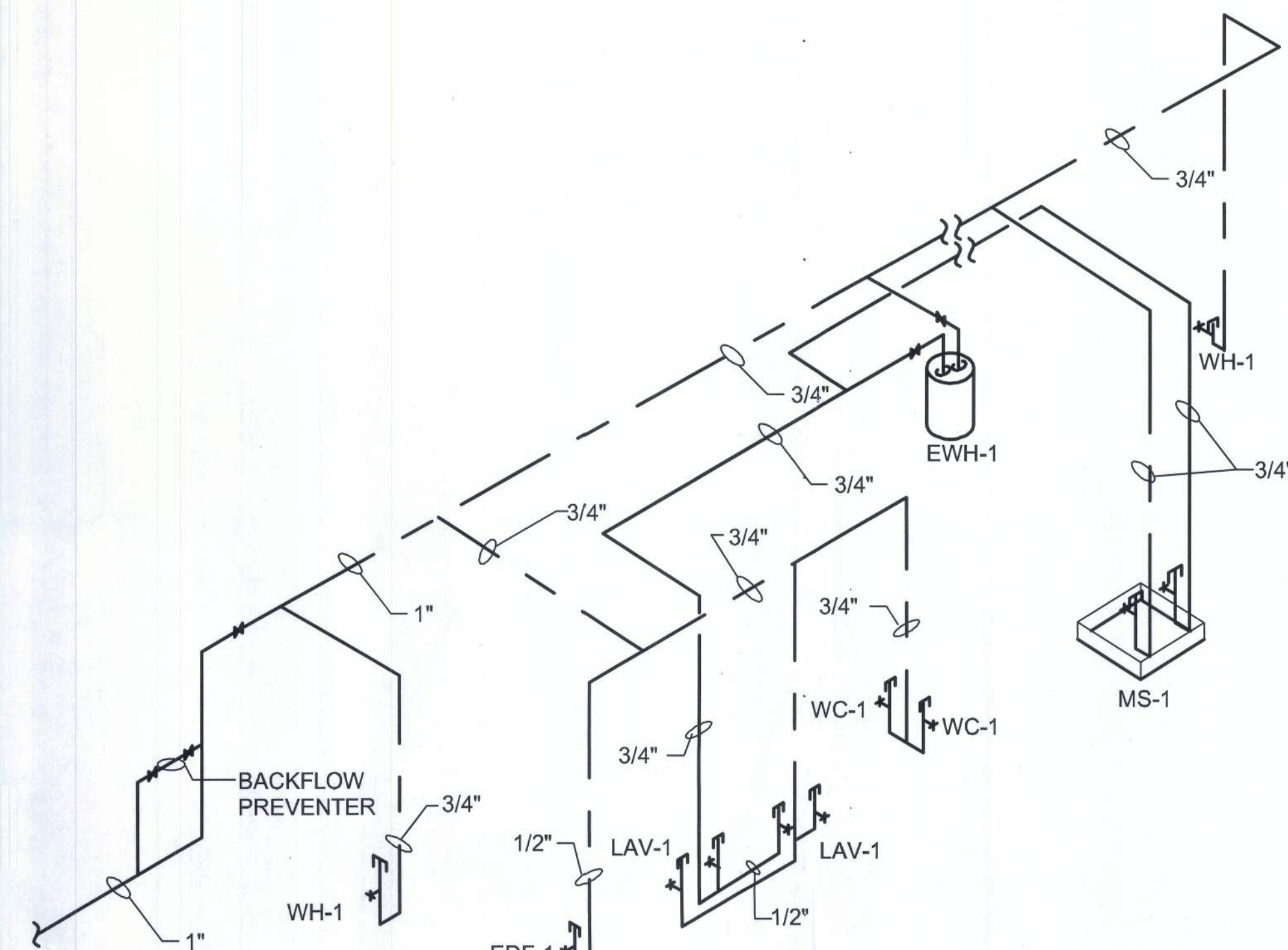
COLD & HOT WATER DIAGRAM SEE SHEET P1.C FOR PLUMBING DEVICE CODES
