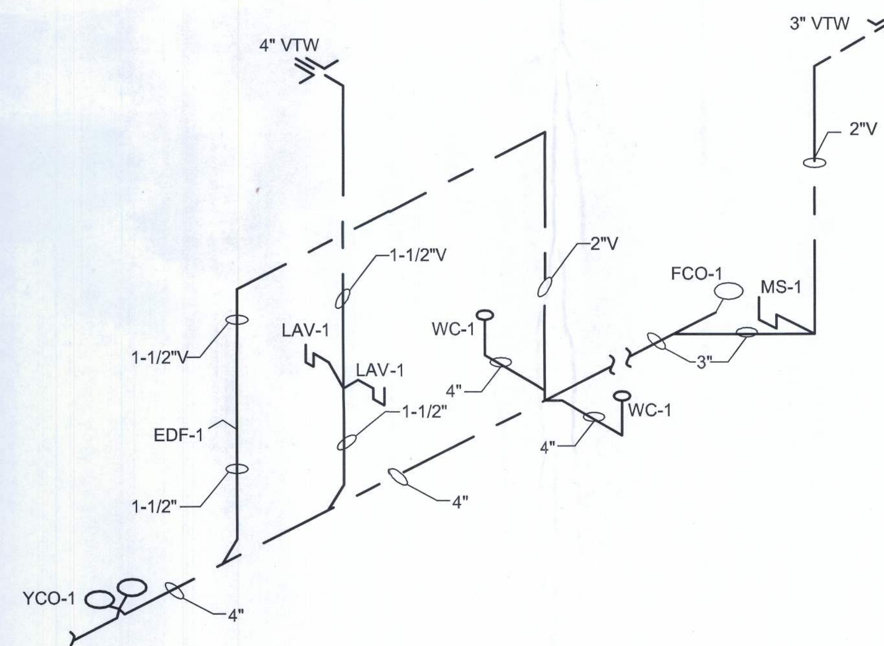
SANITARY & VENT DIAGRAM SEE SHEET P1.C FOR PLUMBING DEVICE CODES
