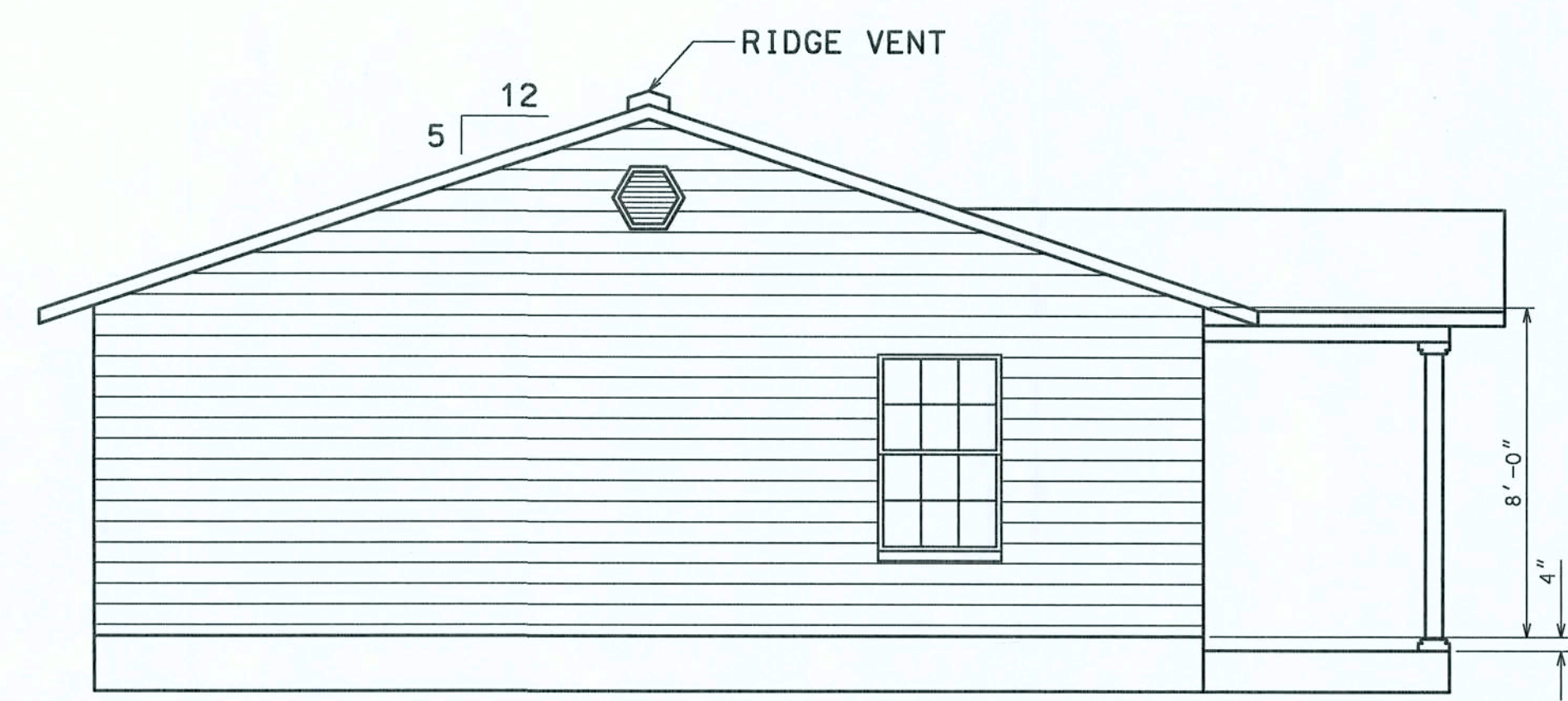
LEFT ELEVATION
