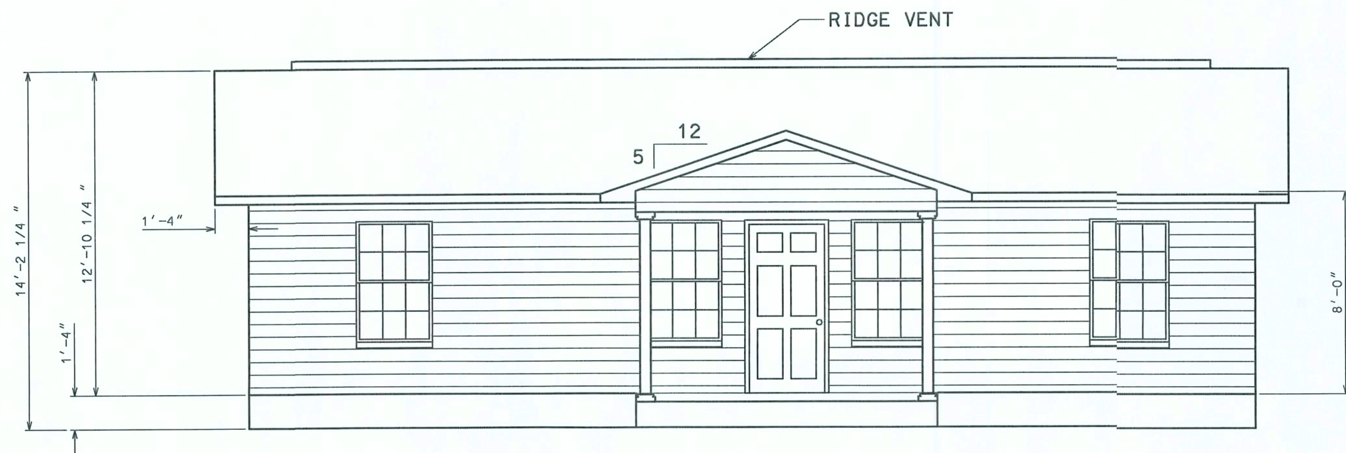
FRONT ELEVATION
