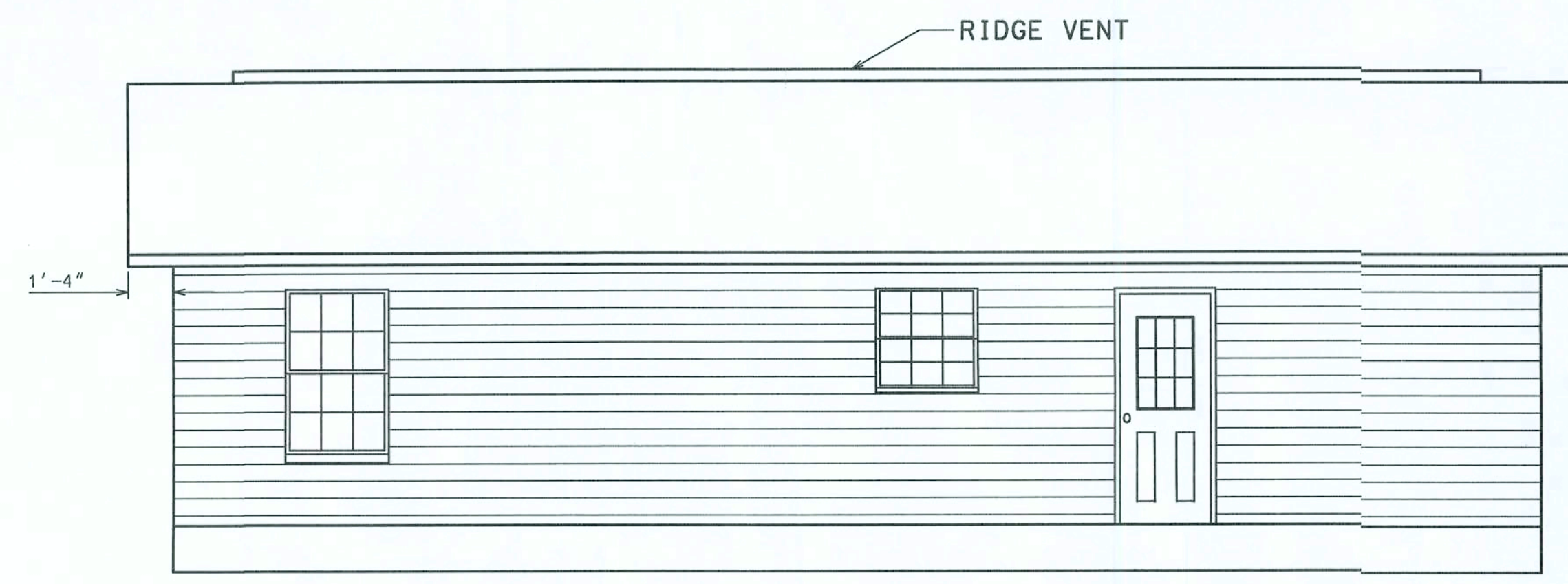
REAR ELEVATION
