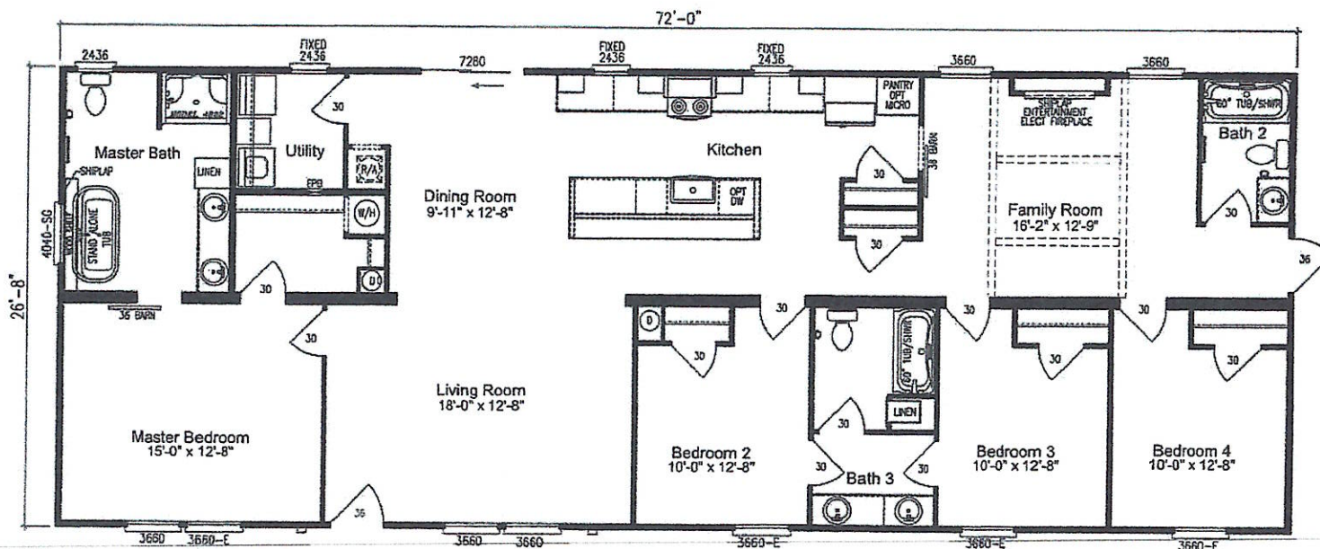
MODEL: 290LY28724A 4 BR. ~ 3 BA. 28'-0" X 72'-0" ~1920 SQ. FT.
