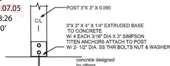
POST TO CONCRETE
