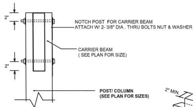
POST/ COLUMN TO BEAM
