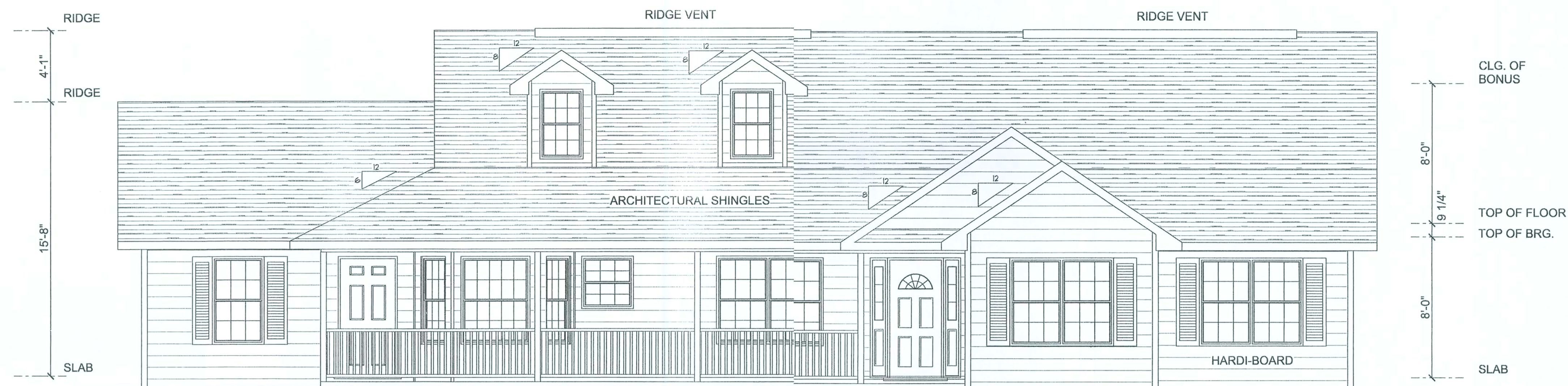
FRONT ELEVATION
