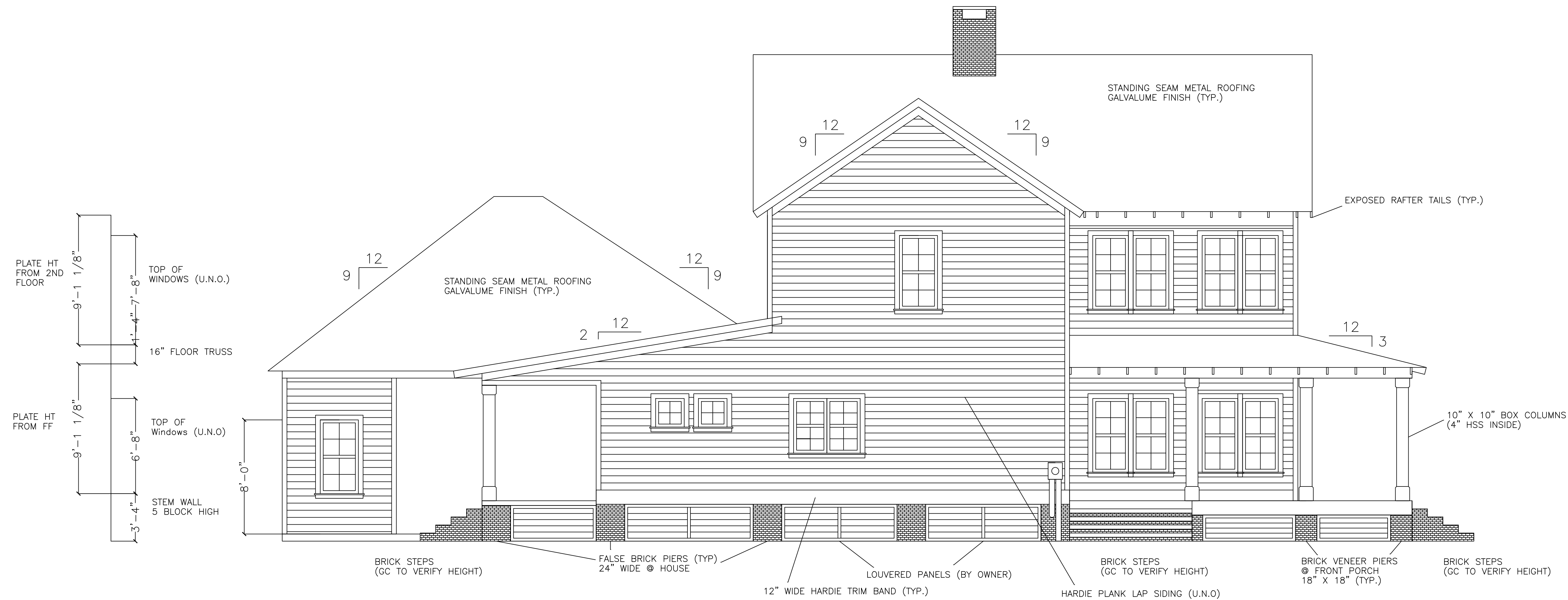
Side/South Elevation
