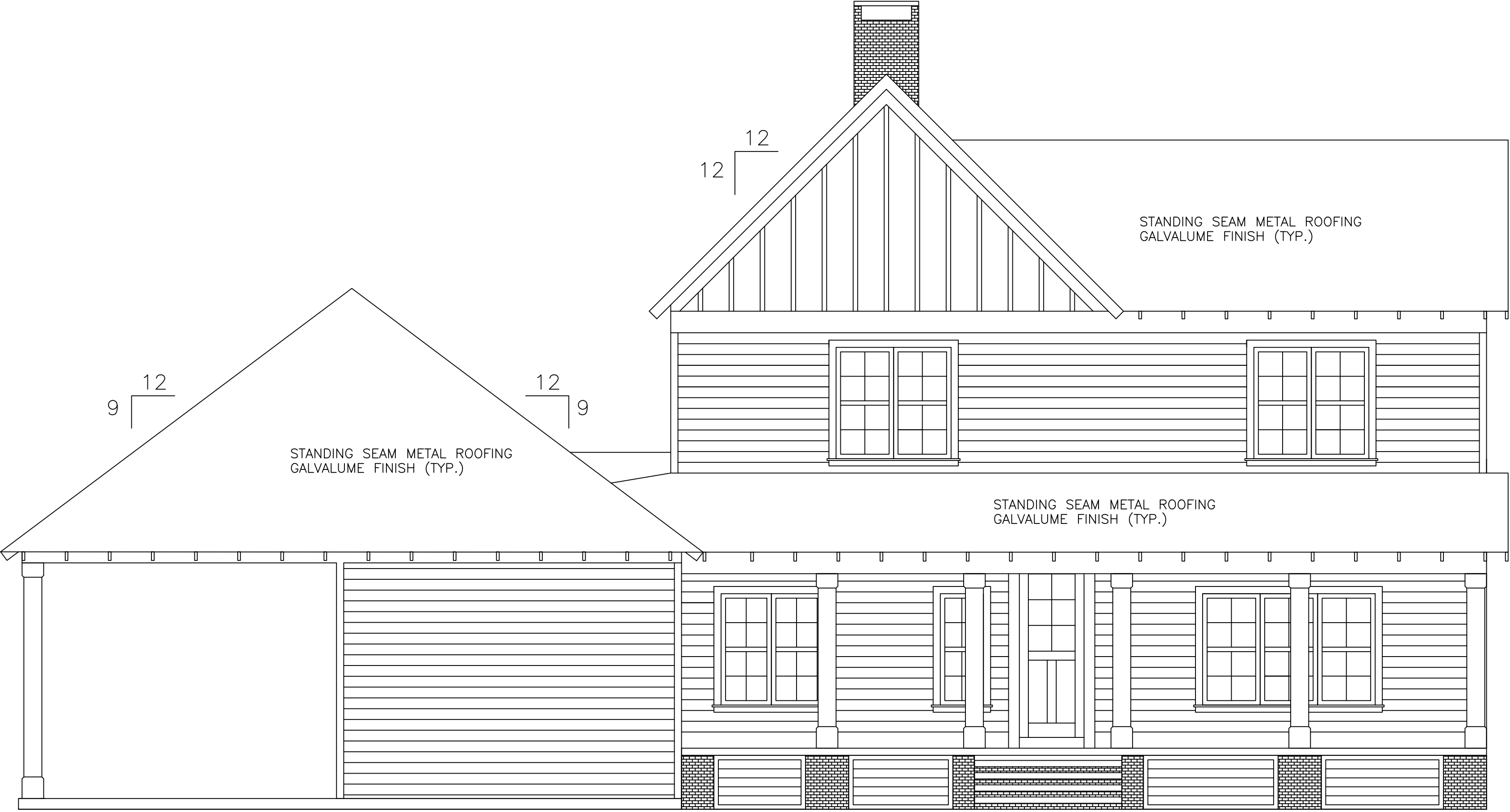
Rear/West Elevation
