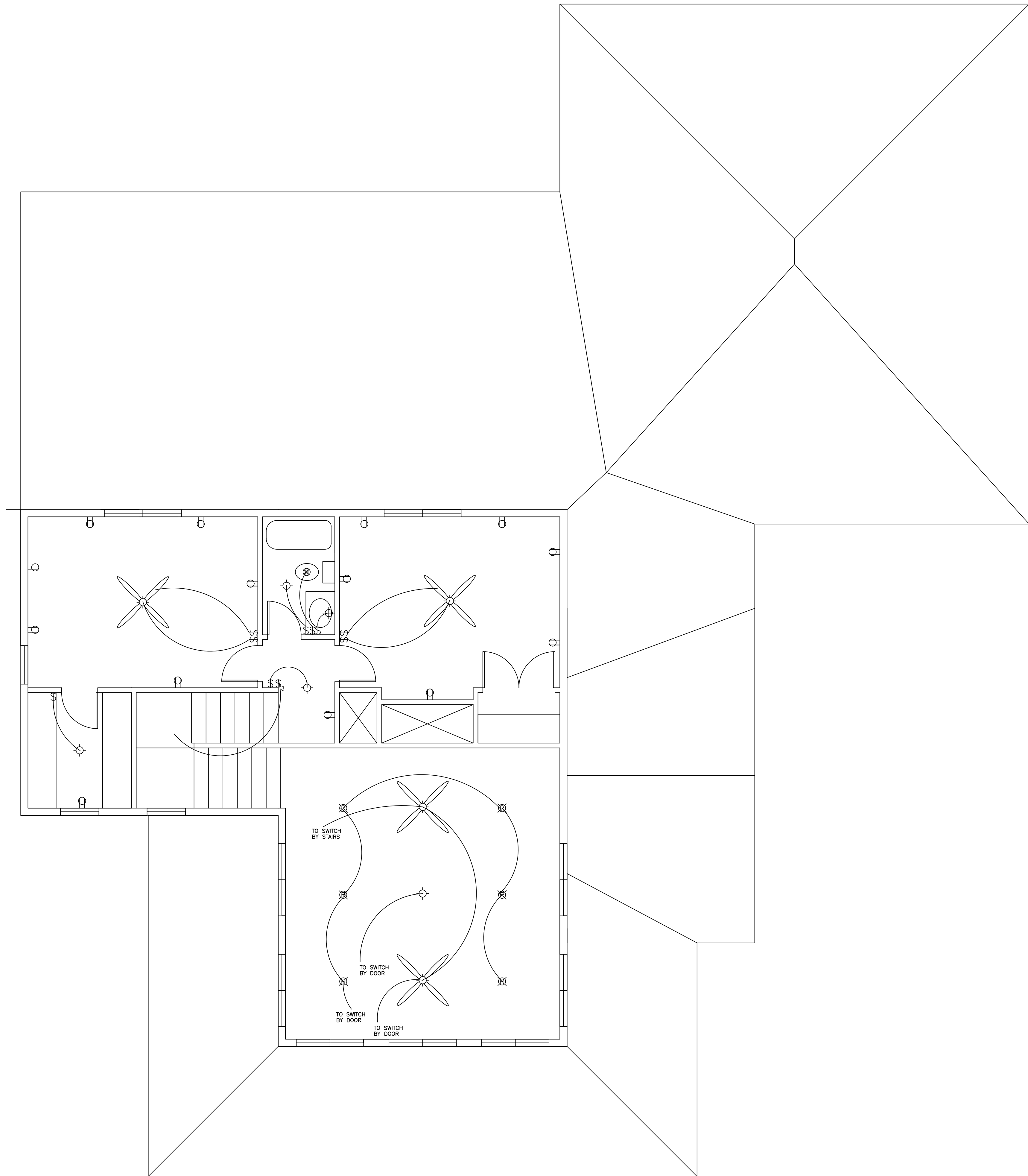
UPPER LEVEL ELECTRICAL PLAN
