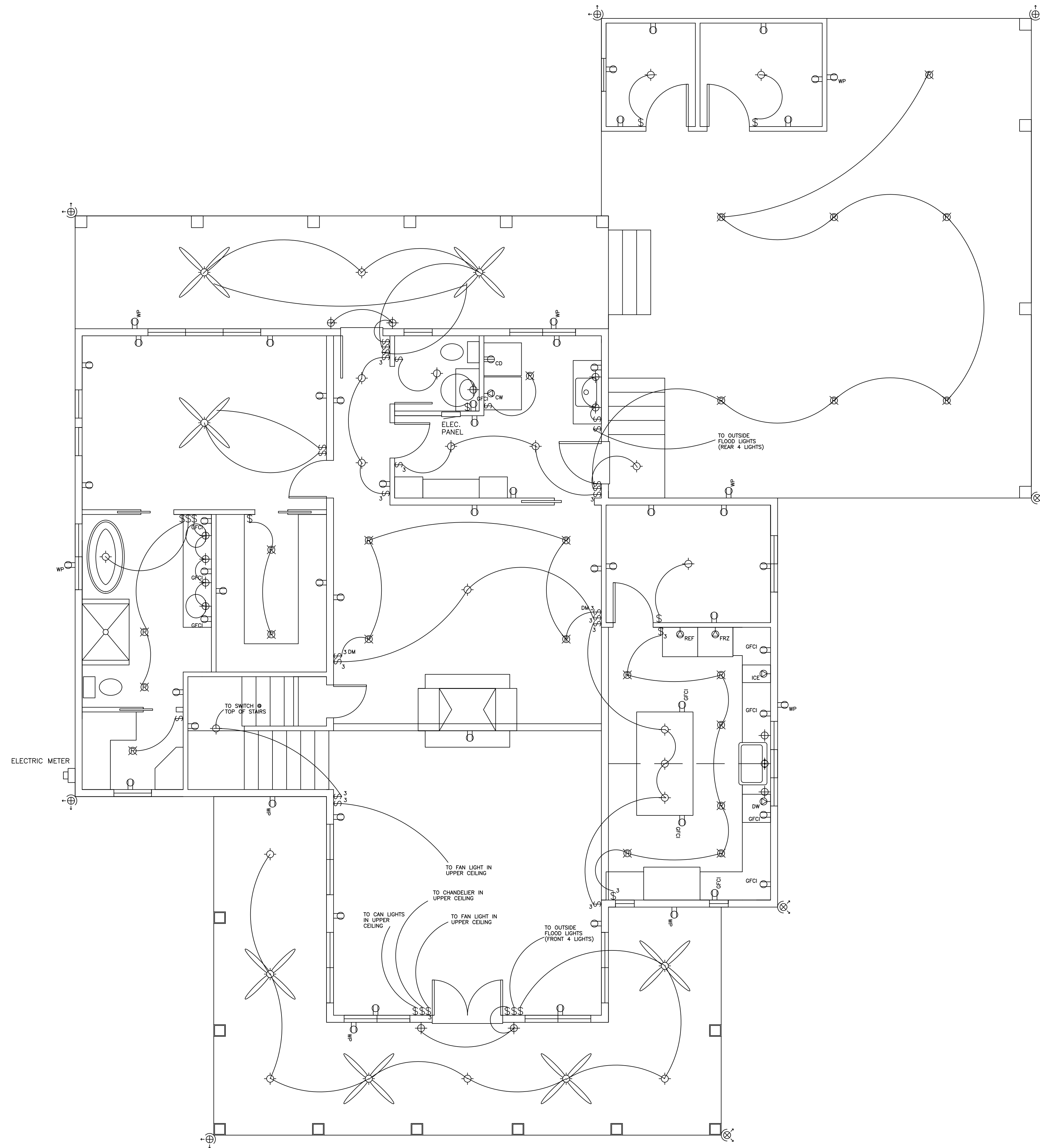
MAIN LEVEL ELECTRICAL PLAN
