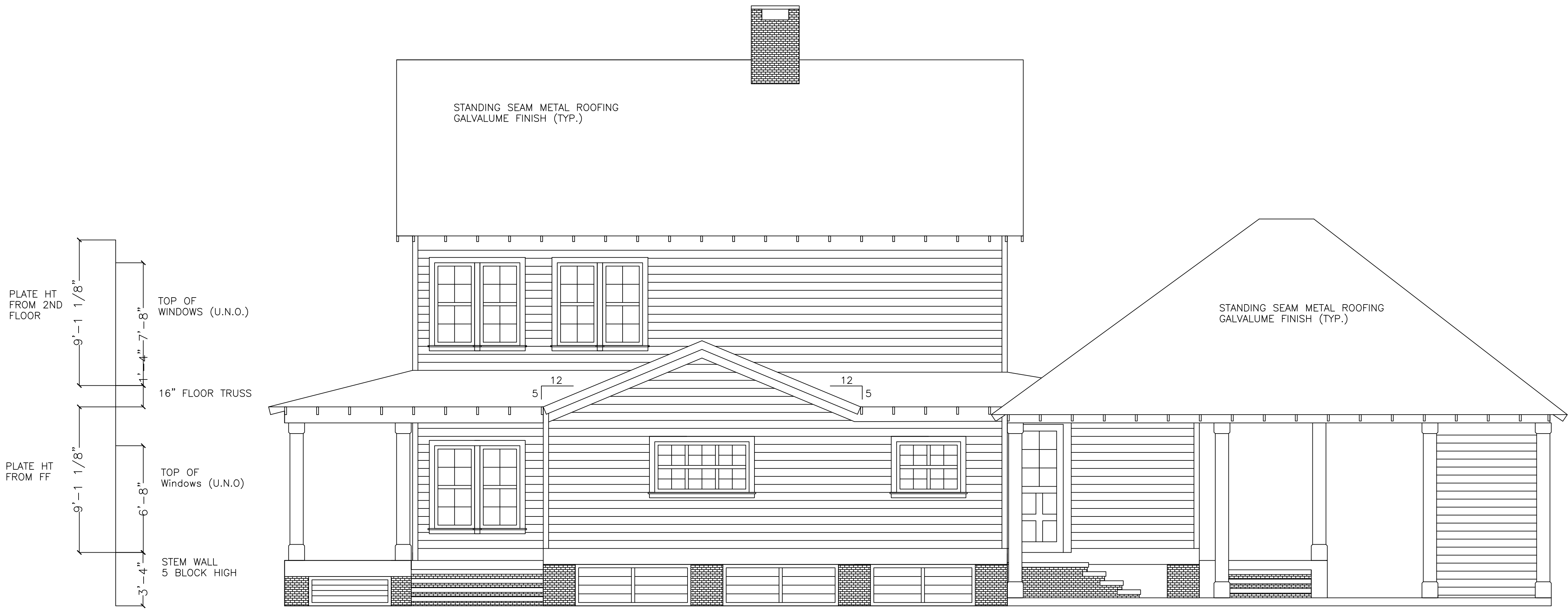
Side/North Elevation
