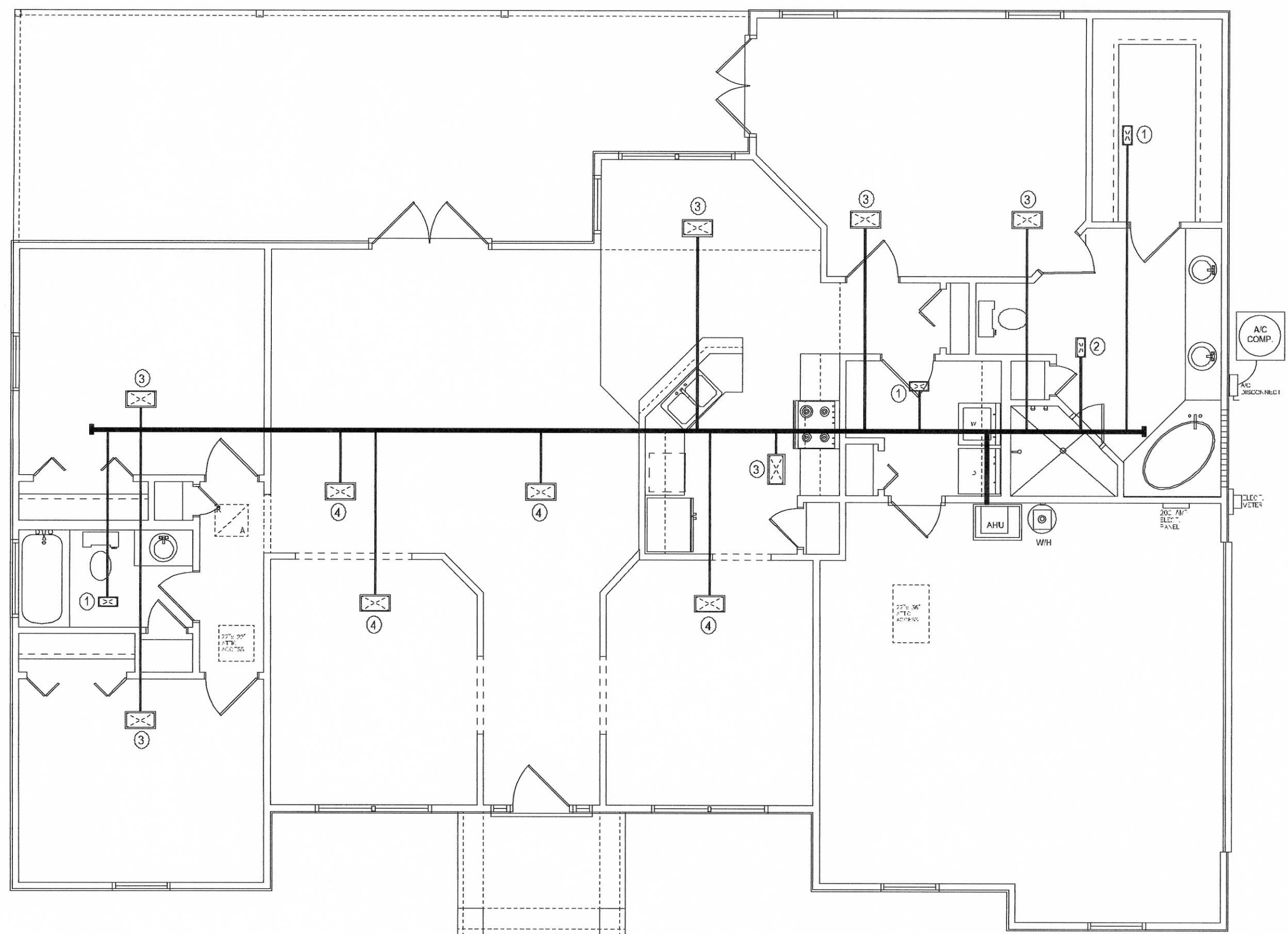
HVAC PLAN SCALE: 3/16" = 1'-0"
