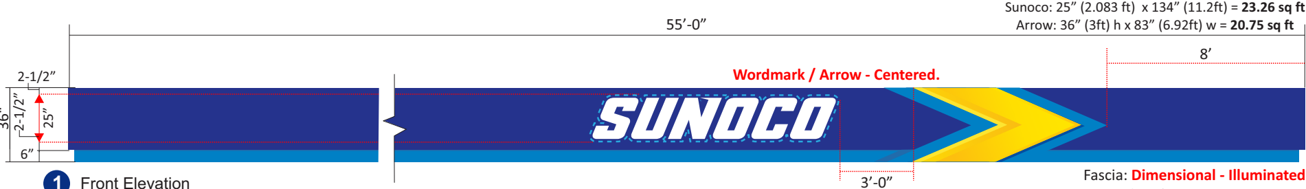
1 Front Elevation
