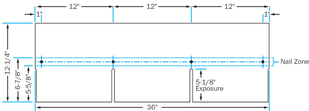
Figure 1. Elite Glass-Seal 4 Nail Pattern (Non-HVHZ only)
