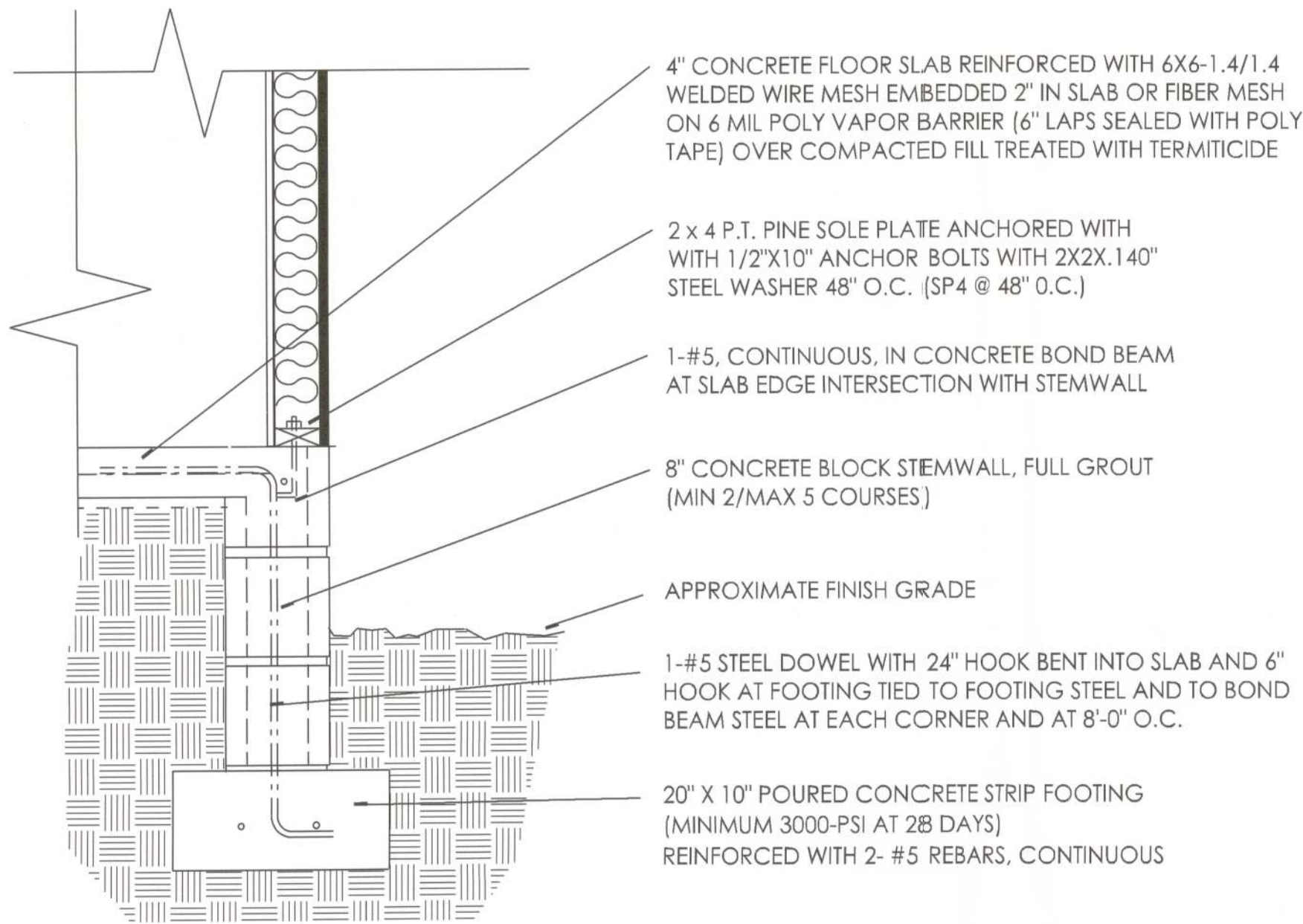
TYPICAL STEMWALL / SECTION A
