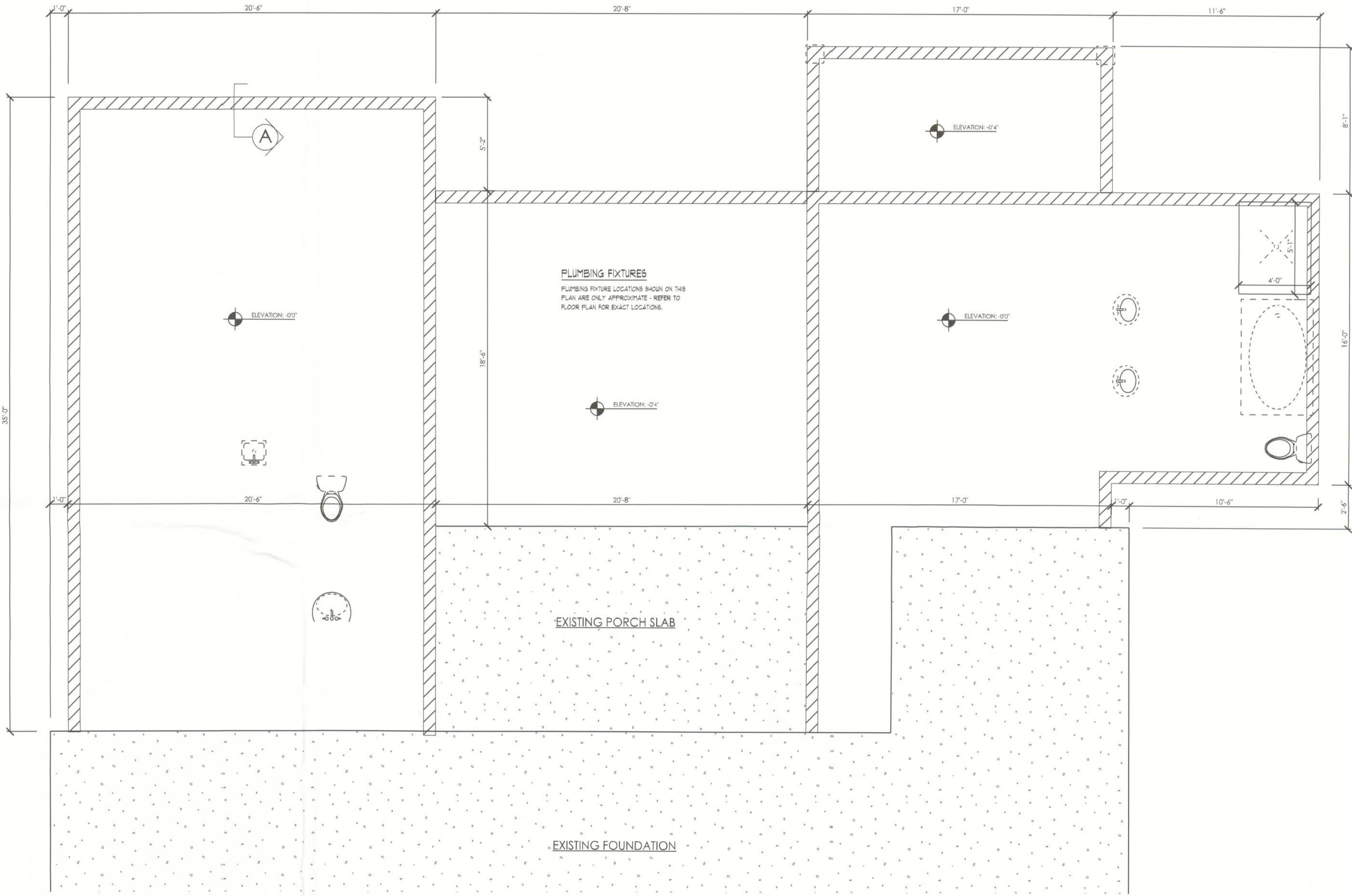
FOUNDATION PLAN SCALE: 1/4" = 1'
