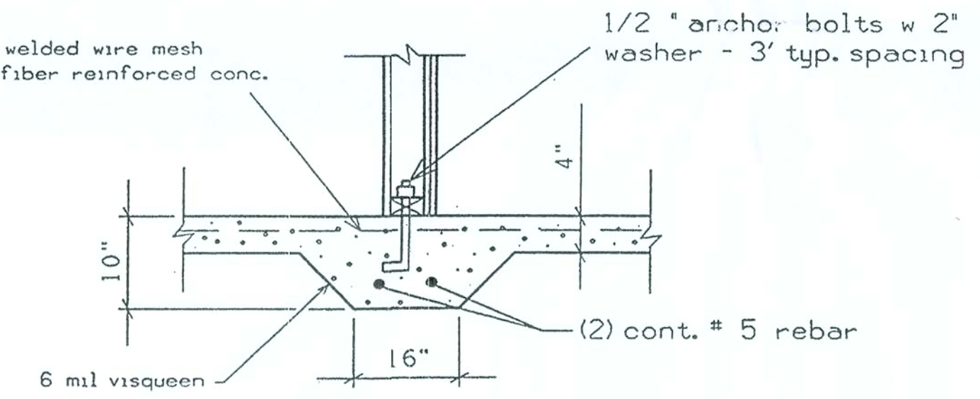
INTERNAL BEARING Interior Wall between Master Bedroom and Sunroom
