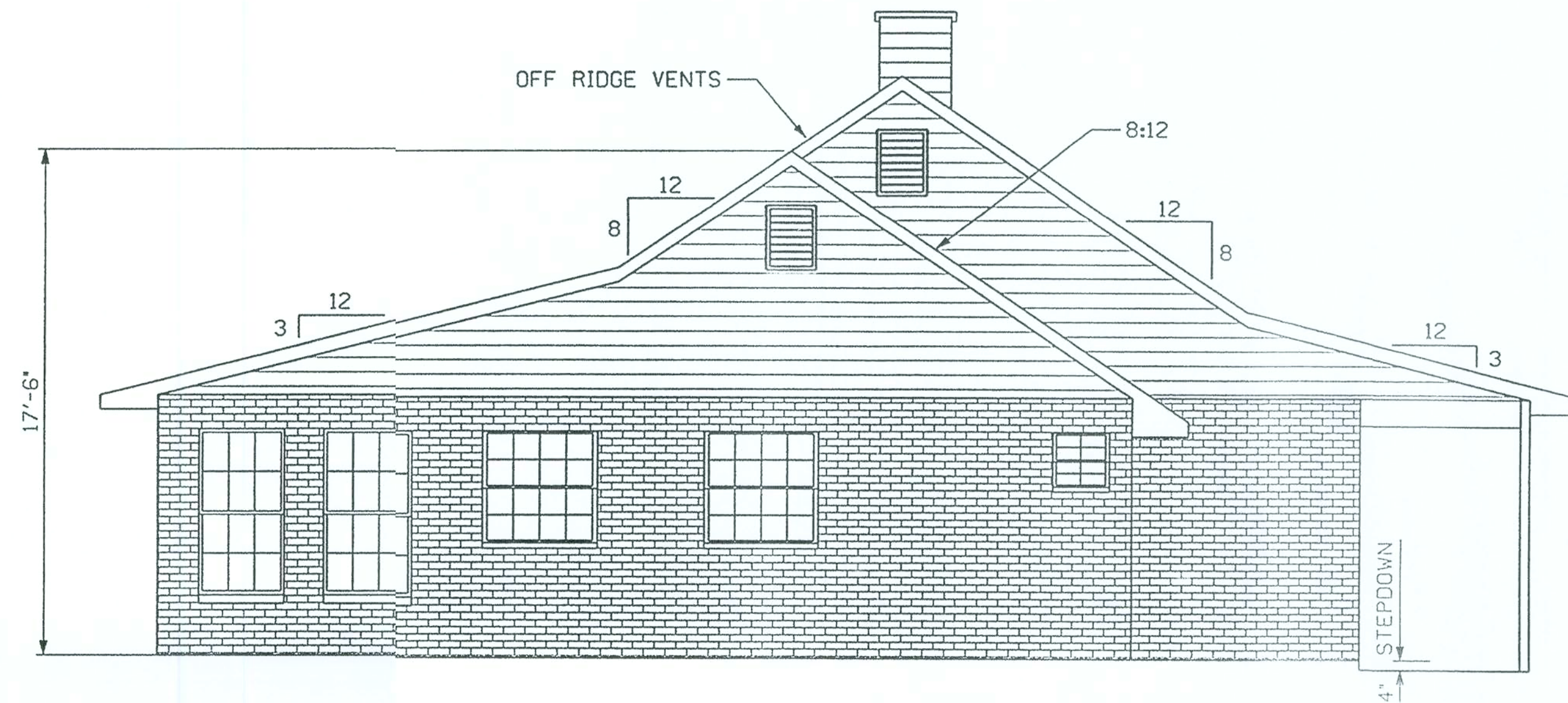
LEFT ELEVATION
