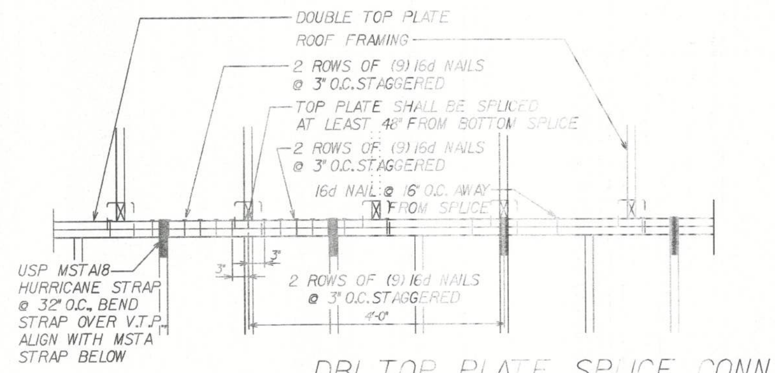
DBL TOP PLATE SPICE CONN.
