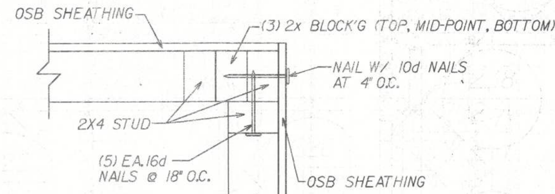
TOP CORNER DETAIL
