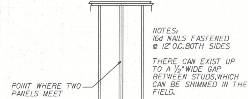
WALL JOINT DETAIL
