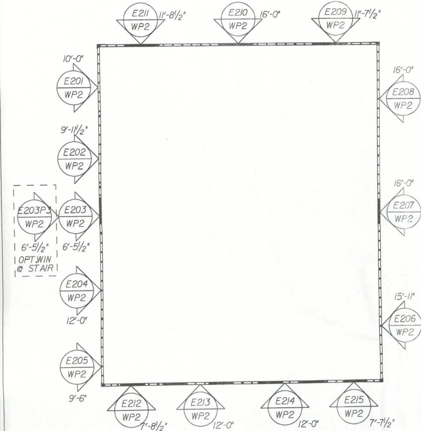
FRONT OF HOUSE SECOND FLOOR PANEL LAYOUT **ELEVATIONS "M" & "V"**
