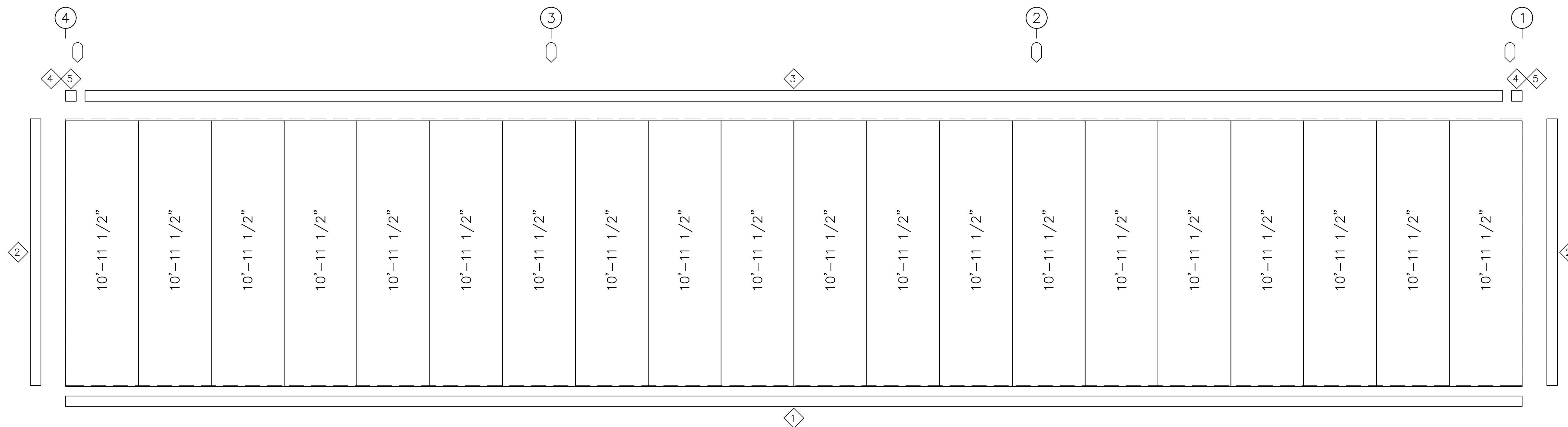
SIDEWALL SHEETING & TRIM: FRAME LINE A
