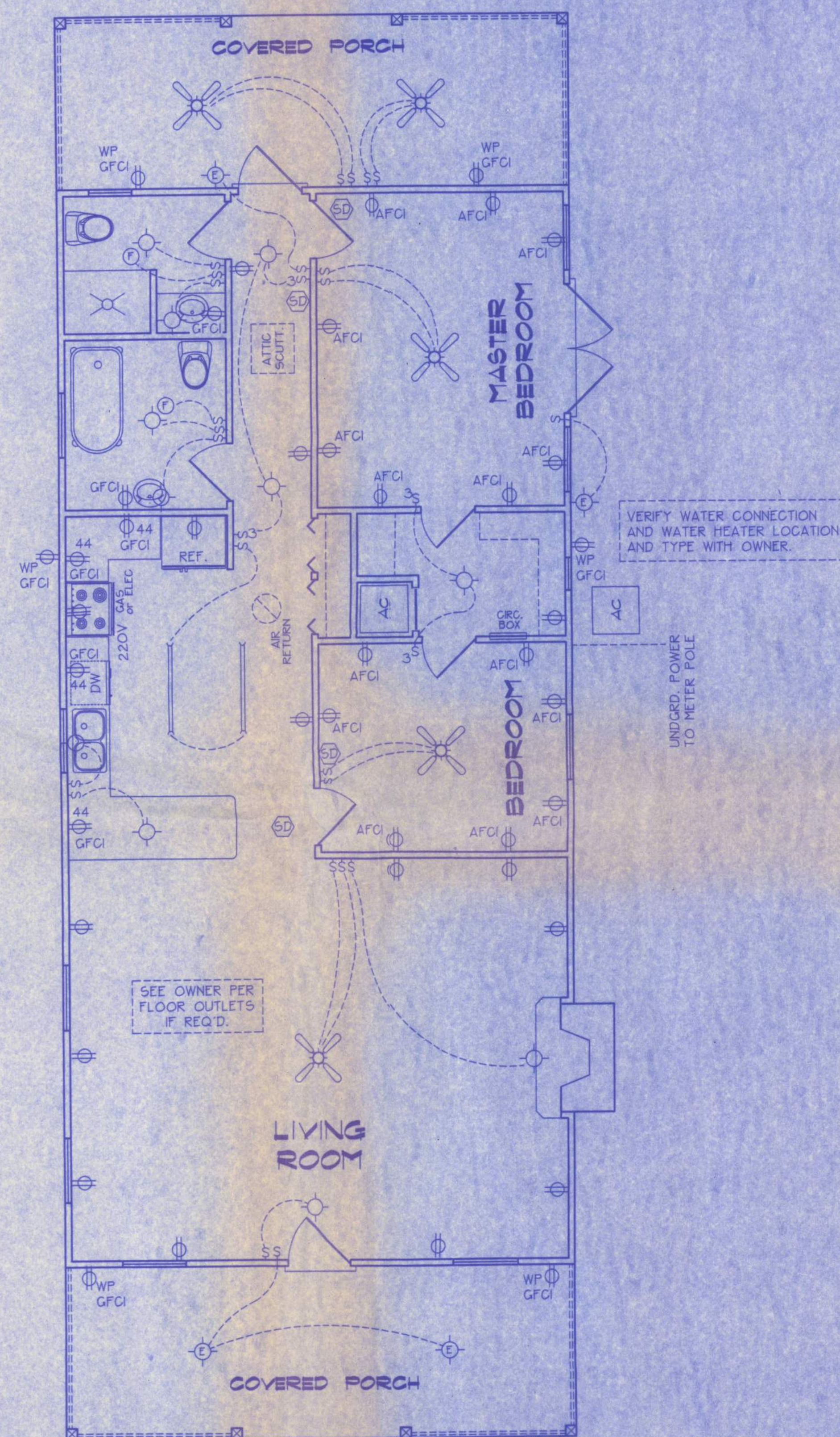
ELECTRICAL PLAN NOT TO SCALE
