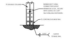
2A RAFTER POST/BASE RAIL CONNECTION DETAIL SCALE: NTS
