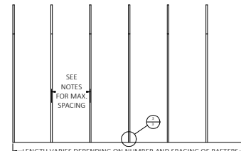
SEE NOTES FOR MAX. SPACING TYPICAL RAFTER/COLUMN SIDE FRAME SECTION
