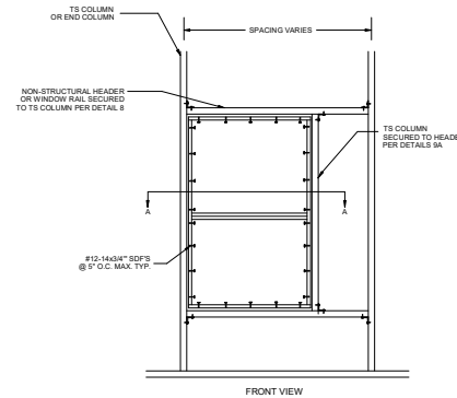
11 WINDOW INSTALLATION DETAILS N.T.S.
