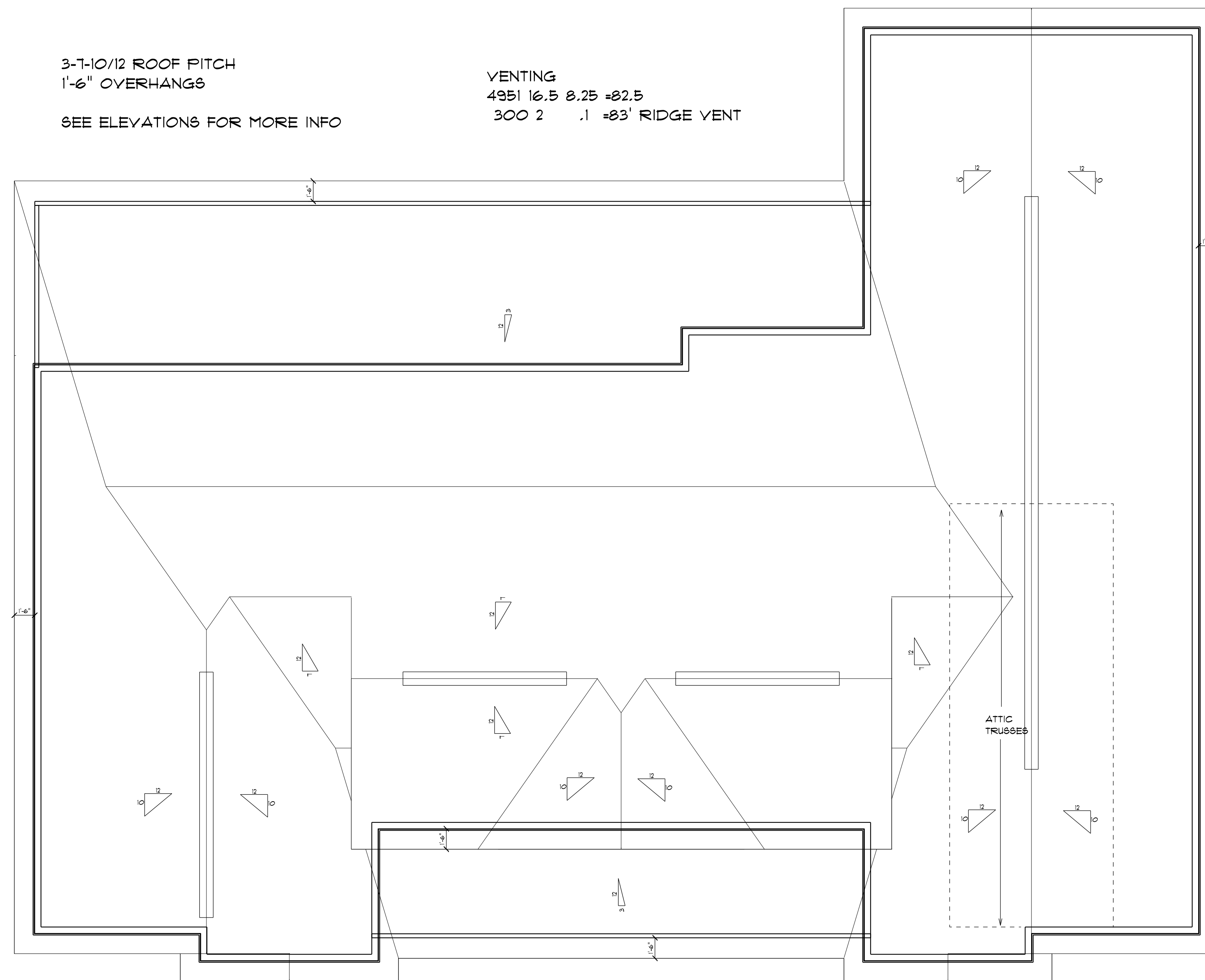
ROOF PLAN
