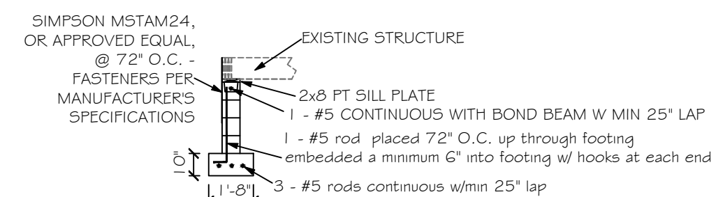
(A) STEM WALL FOUNDATION
