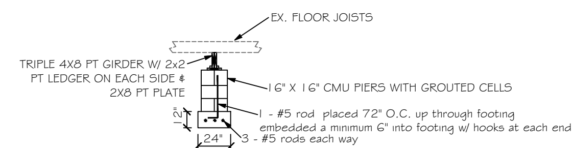
(B) SQUARE PIER (CRAWLSPACE)
