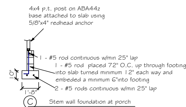
© Stem wall foundation at porch
