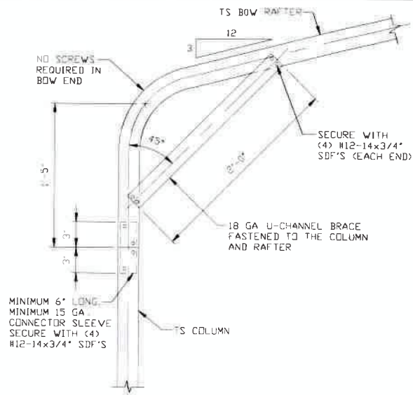
BOX EAVE RAFTER COLUMN CONNECTION DETAIL FOR HEIGHTS \leq 10'-0"
