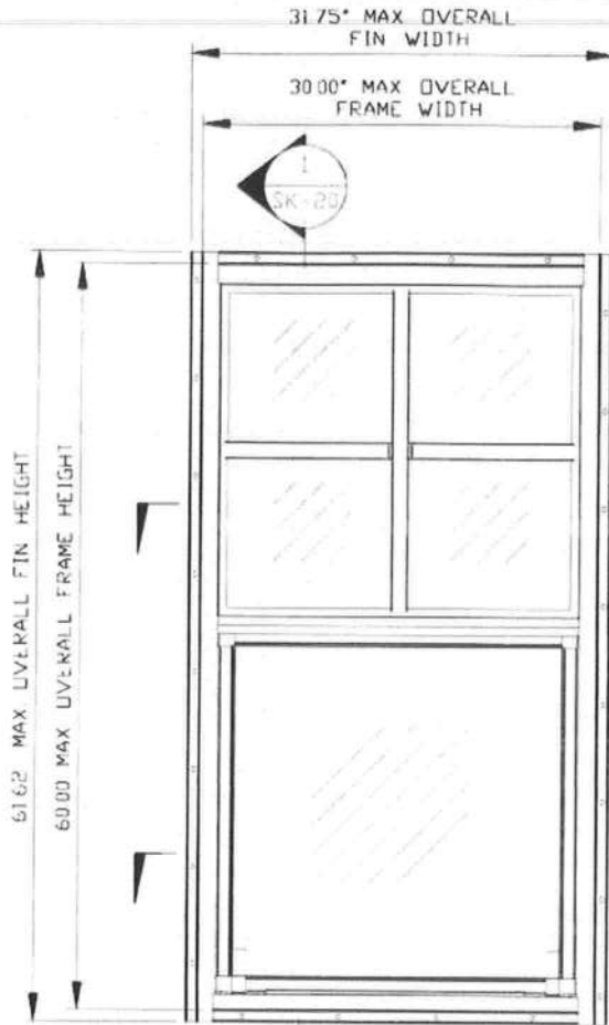
ELEVATION VIEW
