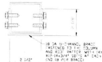
BRACE SECTION
