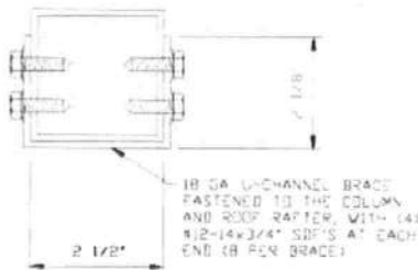
BRACE SECTION
