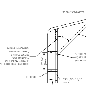
1B BOW EAVE RAFTER COLUMN CONNECTION DETAIL FOR HEIGHTS 16'-0" < TO ≤ 20'-0" SCALE: NTS
