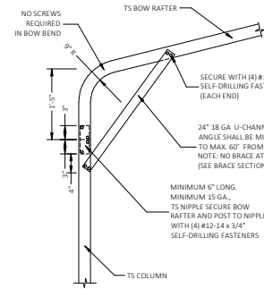
1.2 BOW EAVE RAFTER COLUMN CONNECTION DETAIL FOR HEIGHTS ≤ 12'-0" SCALE: NTS
